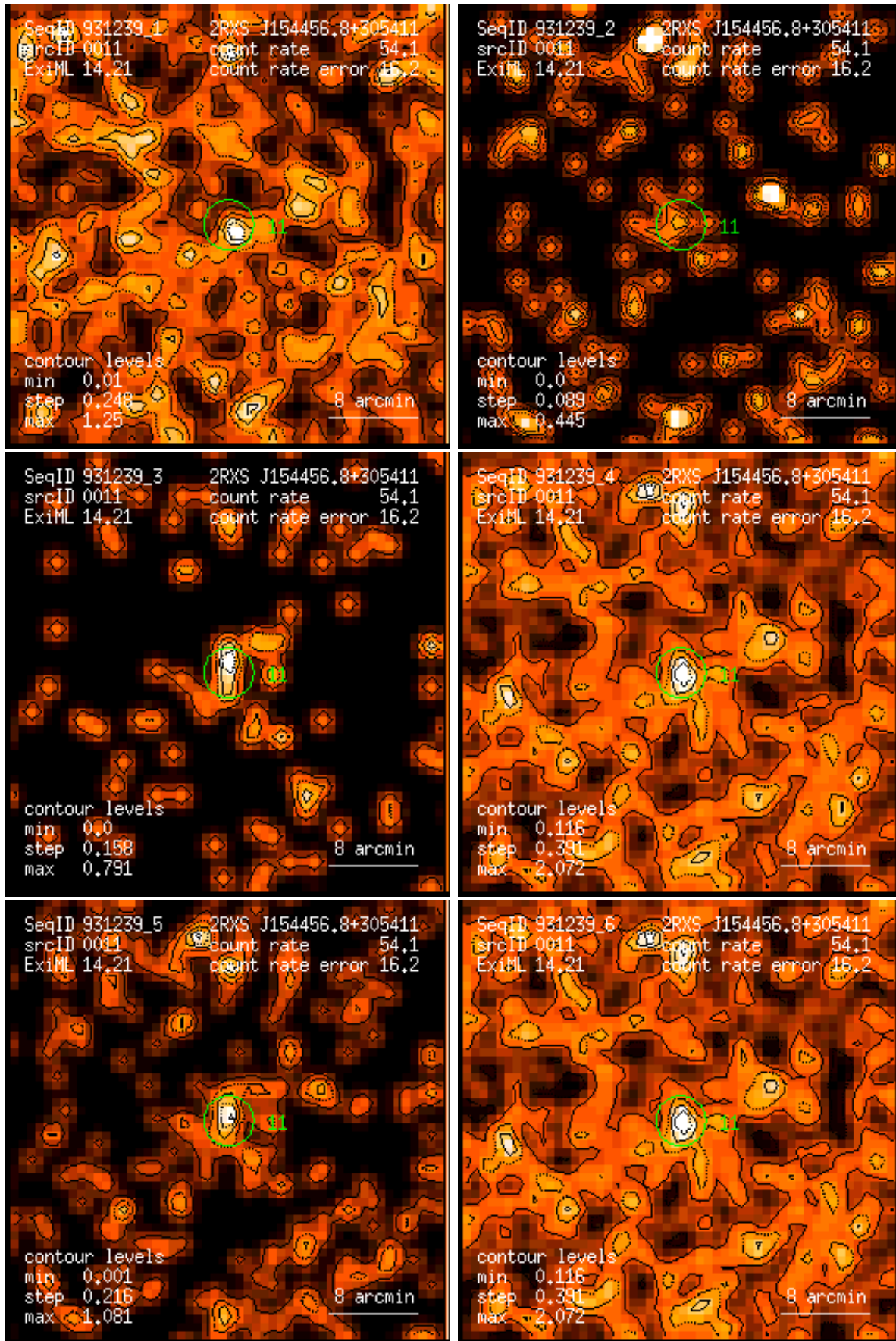
Figure 11: RASS 931239: detection 0011: band rate images, Gaussian filter: (1) PSPC channels 11 – 41, (2) 52 – 90, (3) 91 – 201, (4) 11 – 235, (5) 52 – 201, (6) 11 – 201. Broad band rates in counts/ks. Band rate contour levels in counts/ks/arcmin 2 .
