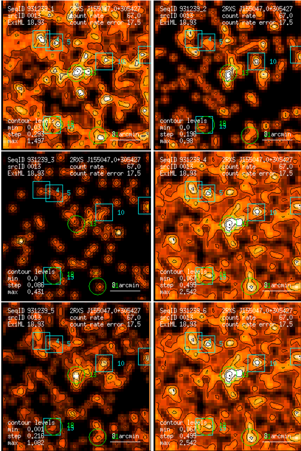
Figure 13: RASS 931239: detection 0013: band rate images, Gaussian filter: (1) PSPC channels 11 – 41, (2) 52 – 90, (3) 91 – 201, (4) 11 – 235, (5) 52 – 201, (6) 11 – 201. Broad band rates in counts/ks. Band rate contour levels in counts/ks/arcmin 2 .
