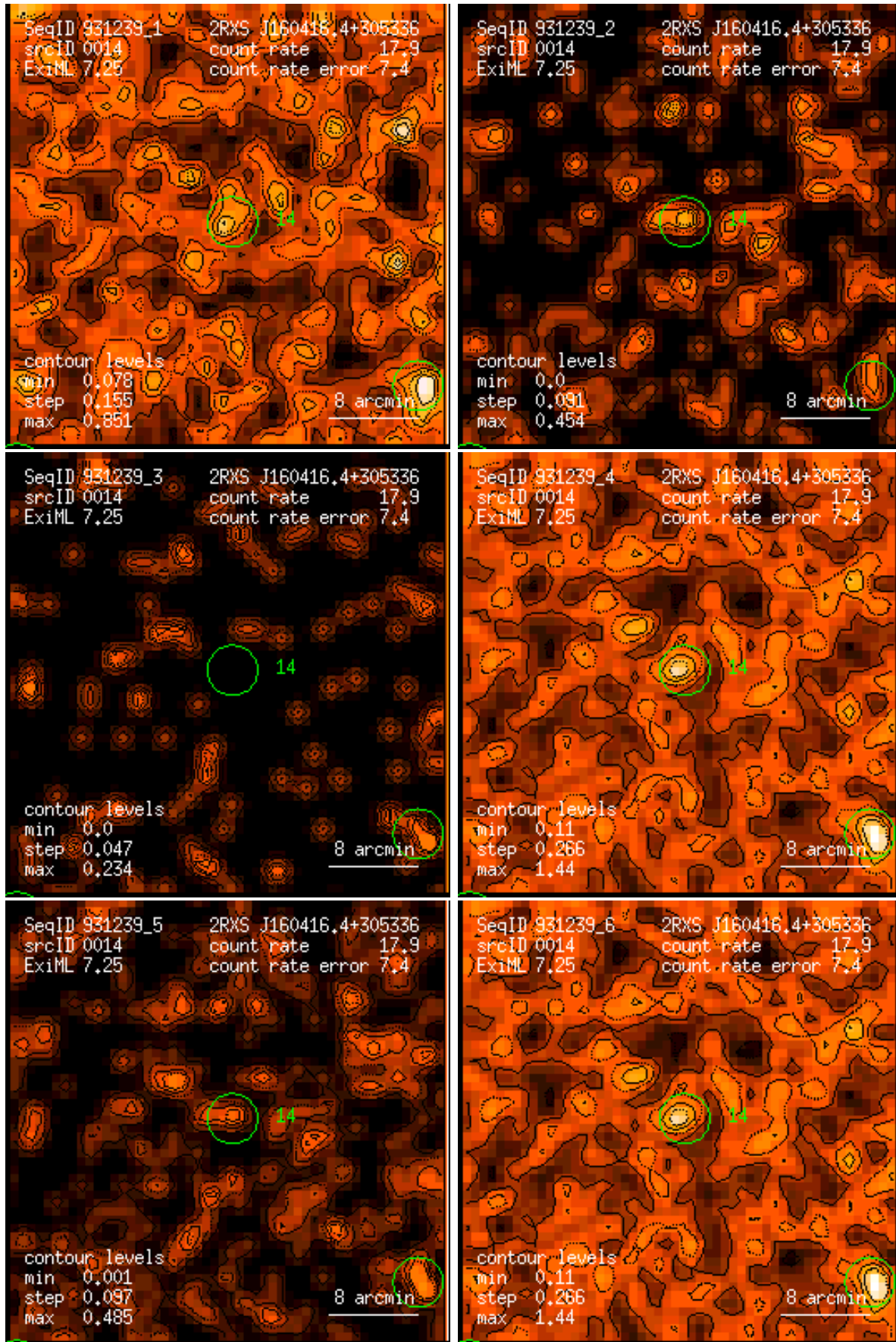
Figure 14: RASS 931239: detection 0014: band rate images, Gaussian filter: (1) PSPC channels 11 – 41, (2) 52 – 90, (3) 91 – 201, (4) 11 – 235, (5) 52 – 201, (6) 11 – 201. Broad band rates in counts/ks. Band rate contour levels in counts/ks/arcmin 2 .
