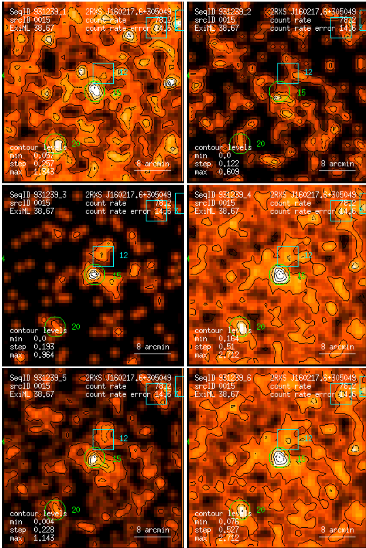
Figure 15: RASS 931239: detection 0015: band rate images, Gaussian filter: (1) PSPC channels 11 – 41, (2) 52 – 90, (3) 91 – 201, (4) 11 – 235, (5) 52 – 201, (6) 11 – 201. Broad band rates in counts/ks. Band rate contour levels in counts/ks/arcmin 2 .
