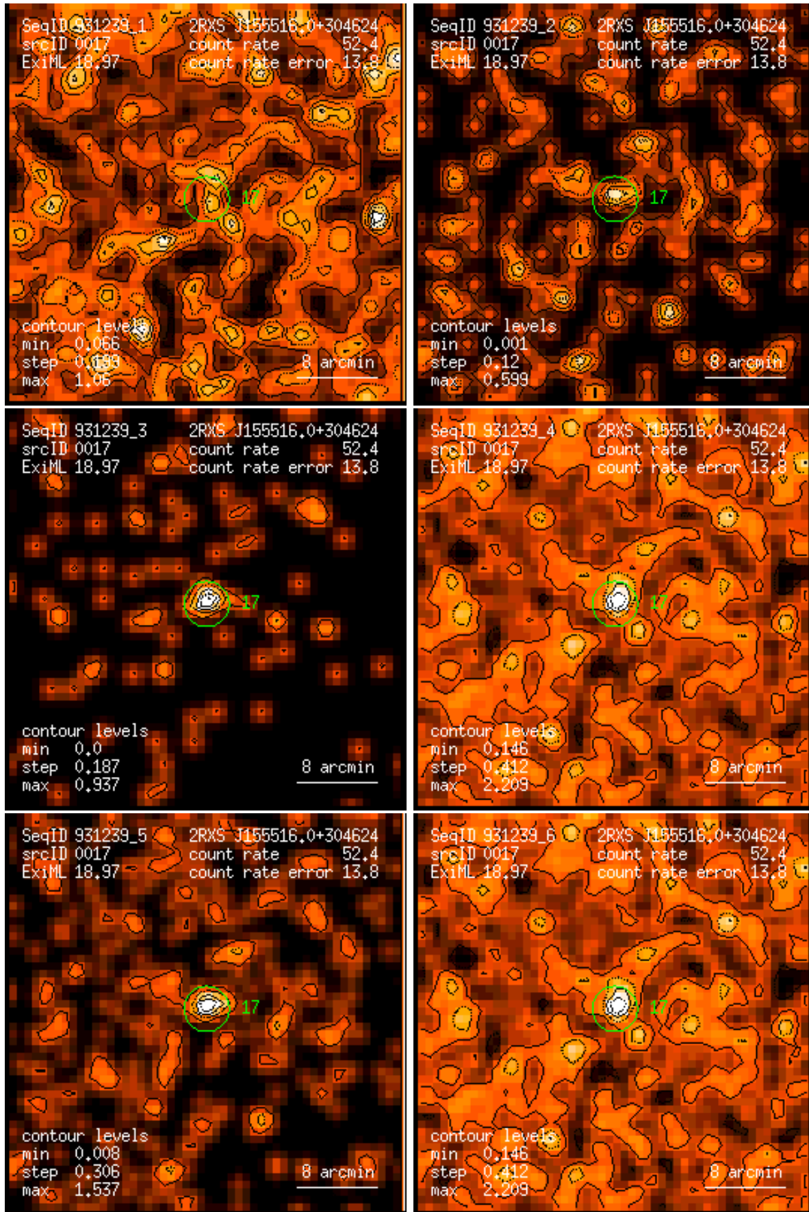
Figure 17: RASS 931239: detection 0017: band rate images, Gaussian filter: (1) PSPC channels 11 – 41, (2) 52 – 90, (3) 91 – 201, (4) 11 – 235, (5) 52 – 201, (6) 11 – 201. Broad band rates in counts/ks. Band rate contour levels in counts/ks/arcmin 2 .
