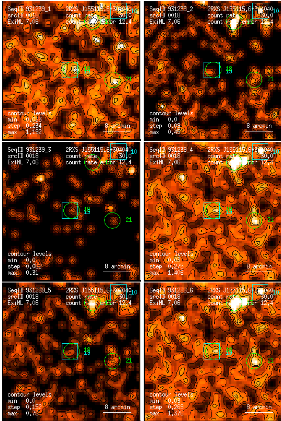
Figure 18: RASS 931239: detection 0018: band rate images, Gaussian filter: (1) PSPC channels 11 – 41, (2) 52 – 90, (3) 91 – 201, (4) 11 – 235, (5) 52 – 201, (6) 11 – 201. Broad band rates in counts/ks. Band rate contour levels in counts/ks/arcmin 2 .
