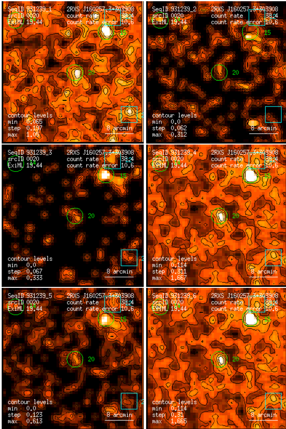
Figure 20: RASS 931239: detection 0020: band rate images, Gaussian filter: (1) PSPC channels 11 – 41, (2) 52 – 90, (3) 91 – 201, (4) 11 – 235, (5) 52 – 201, (6) 11 – 201. Broad band rates in counts/ks. Band rate contour levels in counts/ks/arcmin 2 .
