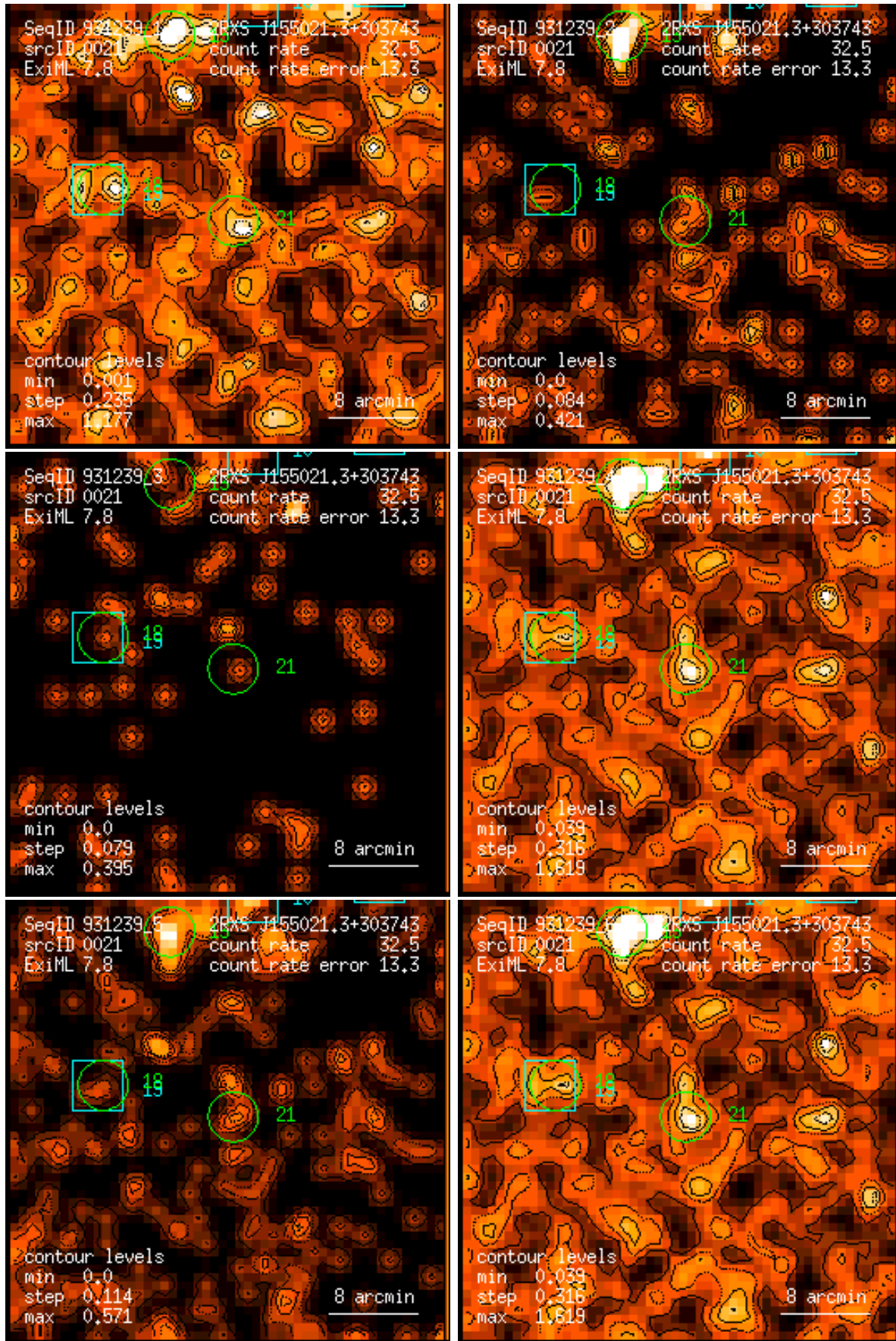
Figure 21: RASS 931239: detection 0021: band rate images, Gaussian filter: (1) PSPC channels 11 – 41, (2) 52 – 90, (3) 91 – 201, (4) 11 – 235, (5) 52 – 201, (6) 11 – 201. Broad band rates in counts/ks. Band rate contour levels in counts/ks/arcmin 2 .
