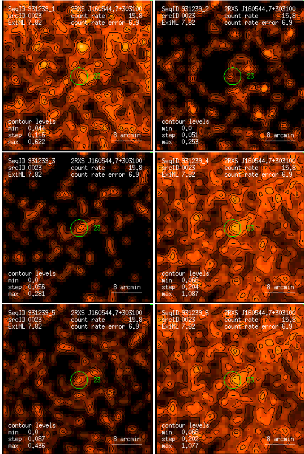
Figure 23: RASS 931239: detection 0023: band rate images, Gaussian filter: (1) PSPC channels 11 – 41, (2) 52 – 90, (3) 91 – 201, (4) 11 – 235, (5) 52 – 201, (6) 11 – 201. Broad band rates in counts/ks. Band rate contour levels in counts/ks/arcmin 2 .
