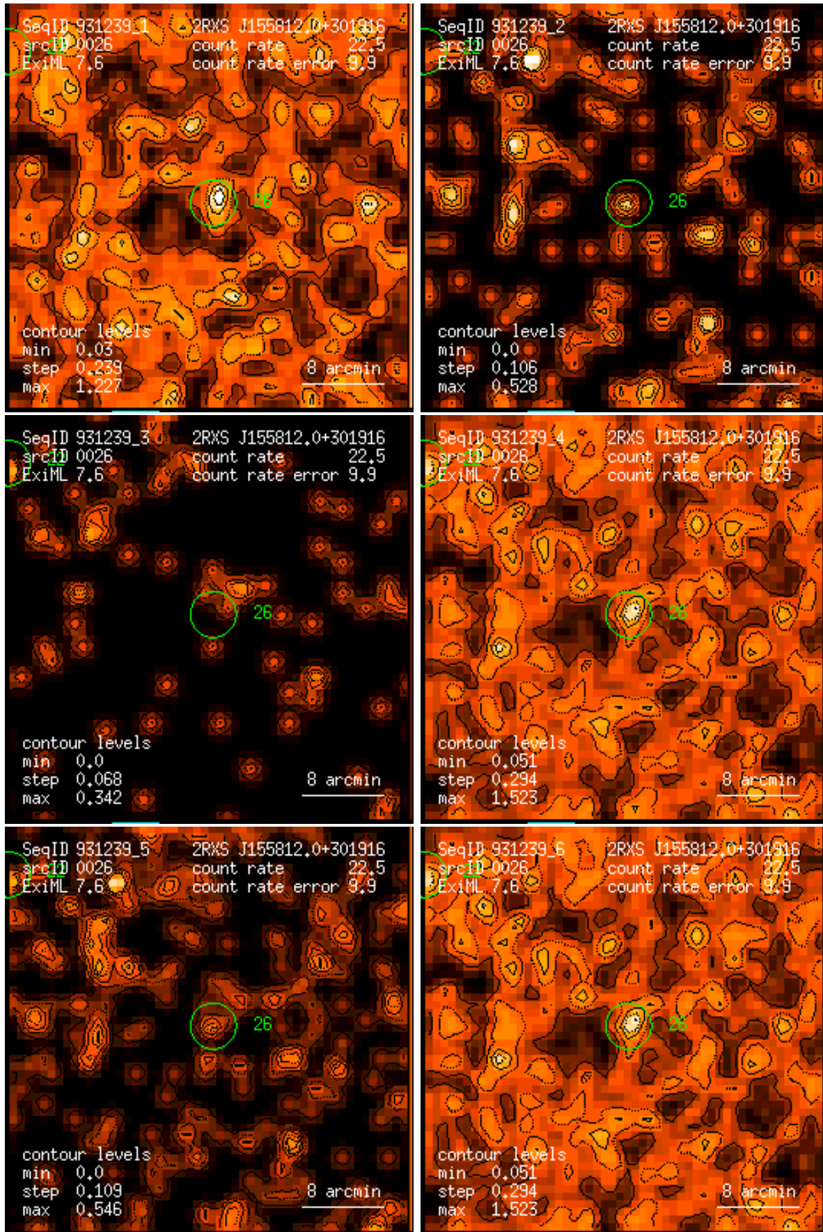
Figure 26: RASS 931239: detection 0026: band rate images, Gaussian filter: (1) PSPC channels 11 – 41, (2) 52 – 90, (3) 91 – 201, (4) 11 – 235, (5) 52 – 201, (6) 11 – 201. Broad band rates in counts/ks. Band rate contour levels in counts/ks/arcmin 2 .
