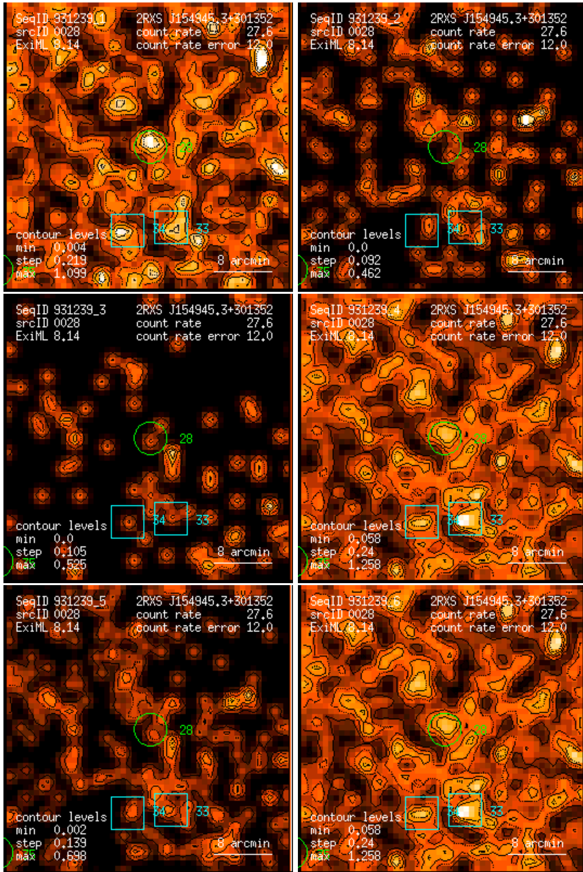
Figure 28: RASS 931239: detection 0028: band rate images, Gaussian filter: (1) PSPC channels 11 – 41, (2) 52 – 90, (3) 91 – 201, (4) 11 – 235, (5) 52 – 201, (6) 11 – 201. Broad band rates in counts/ks. Band rate contour levels in counts/ks/arcmin 2 .
