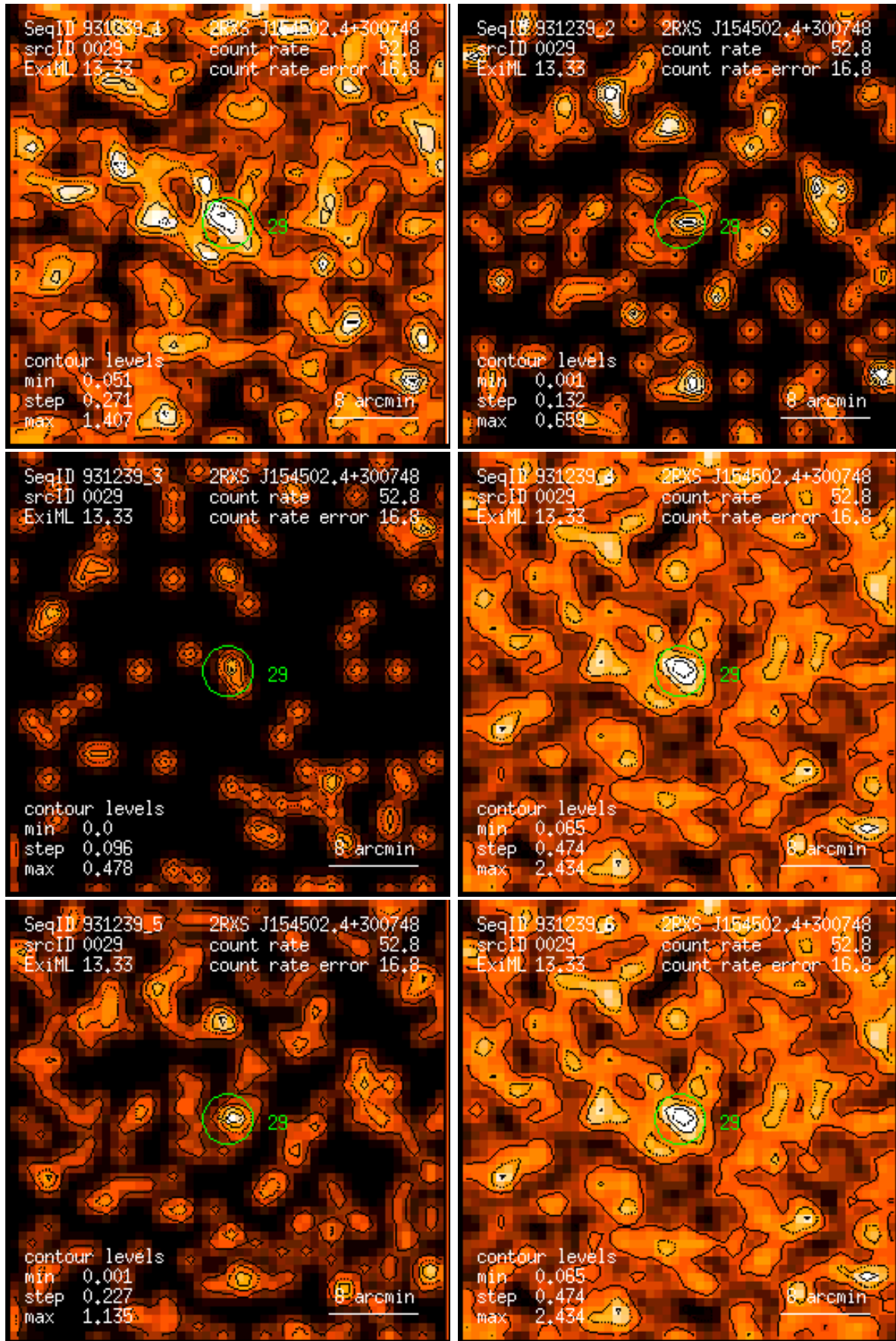
Figure 29: RASS 931239: detection 0029: band rate images, Gaussian filter: (1) PSPC channels 11 – 41, (2) 52 – 90, (3) 91 – 201, (4) 11 – 235, (5) 52 – 201, (6) 11 – 201. Broad band rates in counts/ks. Band rate contour levels in counts/ks/arcmin 2 .
