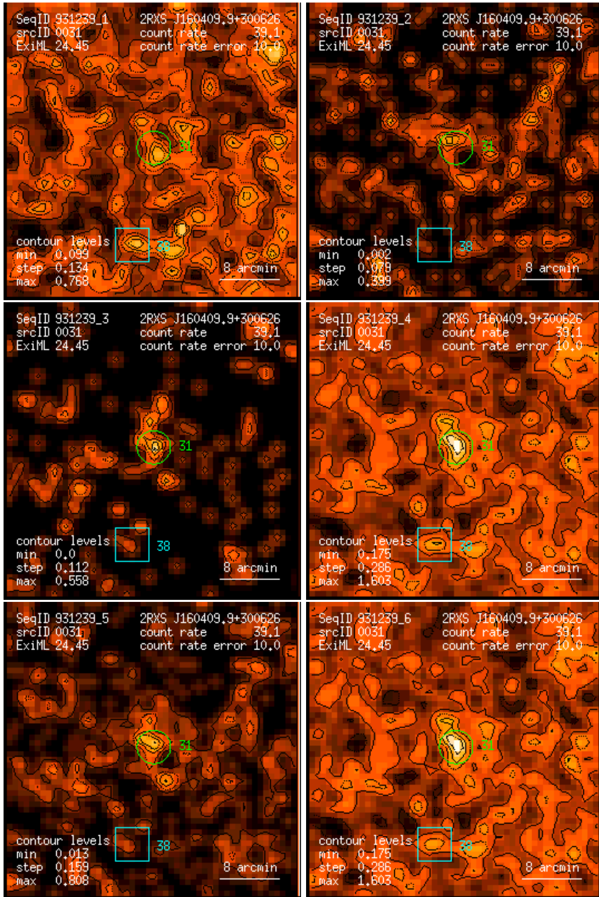
Figure 31: RASS 931239: detection 0031: band rate images, Gaussian filter: (1) PSPC channels 11 – 41, (2) 52 – 90, (3) 91 – 201, (4) 11 – 235, (5) 52 – 201, (6) 11 – 201. Broad band rates in counts/ks. Band rate contour levels in counts/ks/arcmin 2 .
