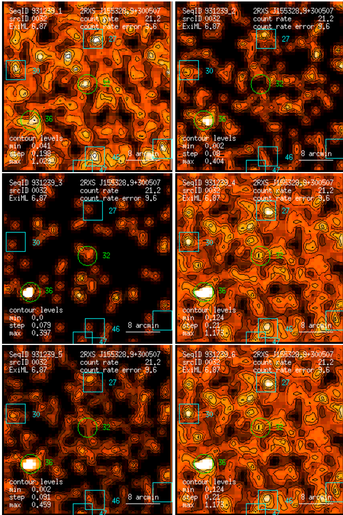
Figure 32: RASS 931239: detection 0032: band rate images, Gaussian filter: (1) PSPC channels 11 – 41, (2) 52 – 90, (3) 91 – 201, (4) 11 – 235, (5) 52 – 201, (6) 11 – 201. Broad band rates in counts/ks. Band rate contour levels in counts/ks/arcmin 2 .
