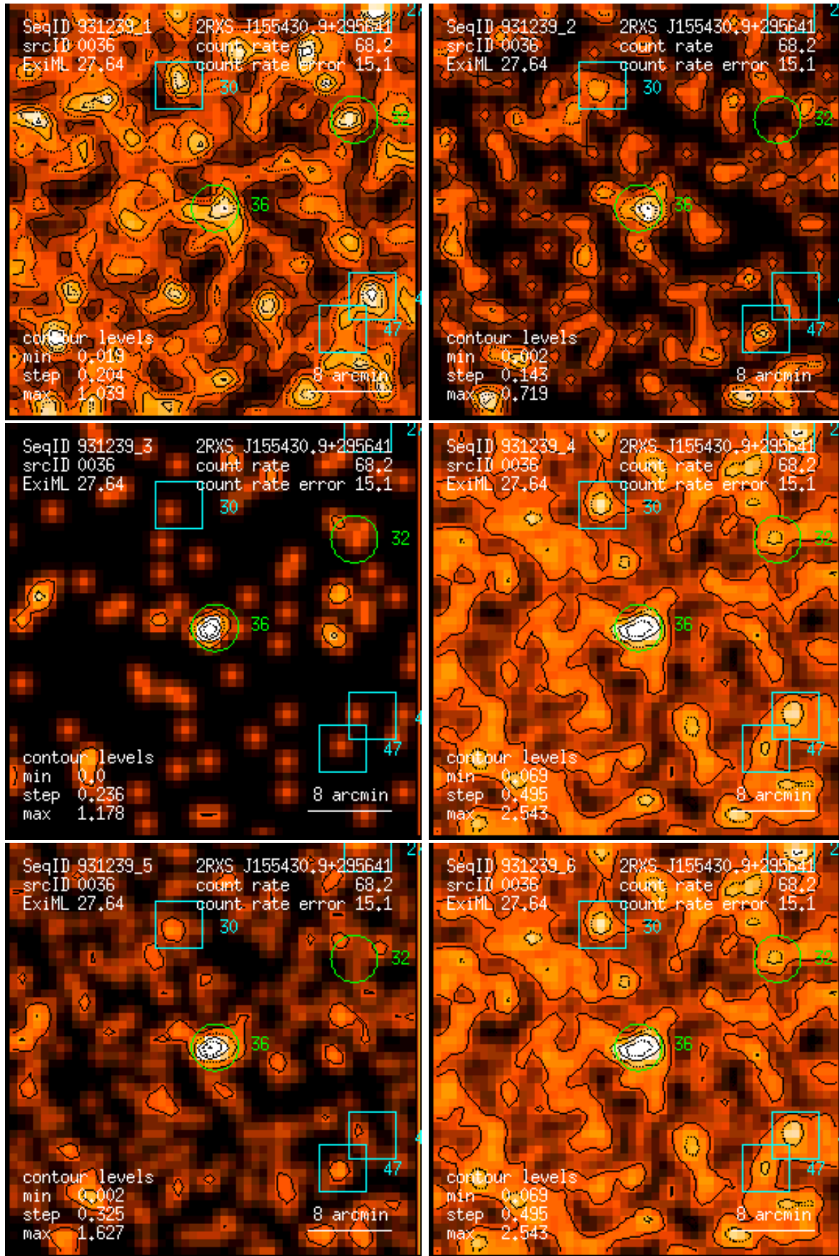
Figure 36: RASS 931239: detection 0036: band rate images, Gaussian filter: (1) PSPC channels 11 – 41, (2) 52 – 90, (3) 91 – 201, (4) 11 – 235, (5) 52 – 201, (6) 11 – 201. Broad band rates in counts/ks. Band rate contour levels in counts/ks/arcmin 2 .
