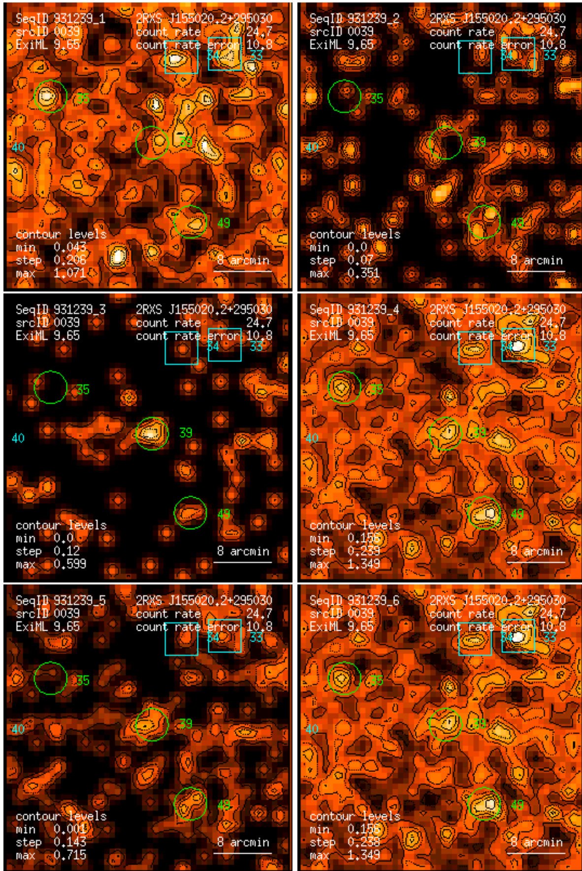
Figure 39: RASS 931239: detection 0039: band rate images, Gaussian filter: (1) PSPC channels 11 – 41, (2) 52 – 90, (3) 91 – 201, (4) 11 – 235, (5) 52 – 201, (6) 11 – 201. Broad band rates in counts/ks. Band rate contour levels in counts/ks/arcmin 2 .
