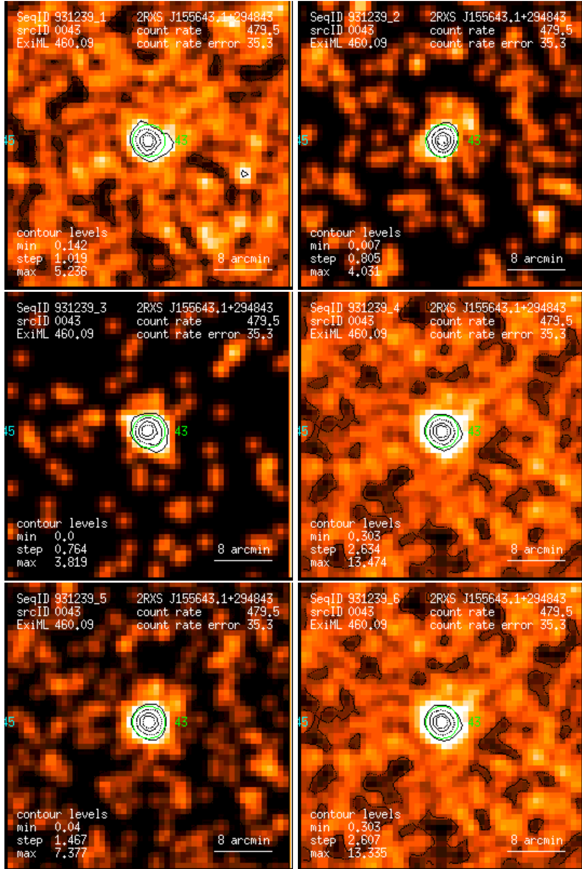
Figure 43: RASS 931239: detection 0043: band rate images, Gaussian filter: (1) PSPC channels 11 – 41, (2) 52 – 90, (3) 91 – 201, (4) 11 – 235, (5) 52 – 201, (6) 11 – 201. Broad band rates in counts/ks. Band rate contour levels in counts/ks/arcmin 2 .
