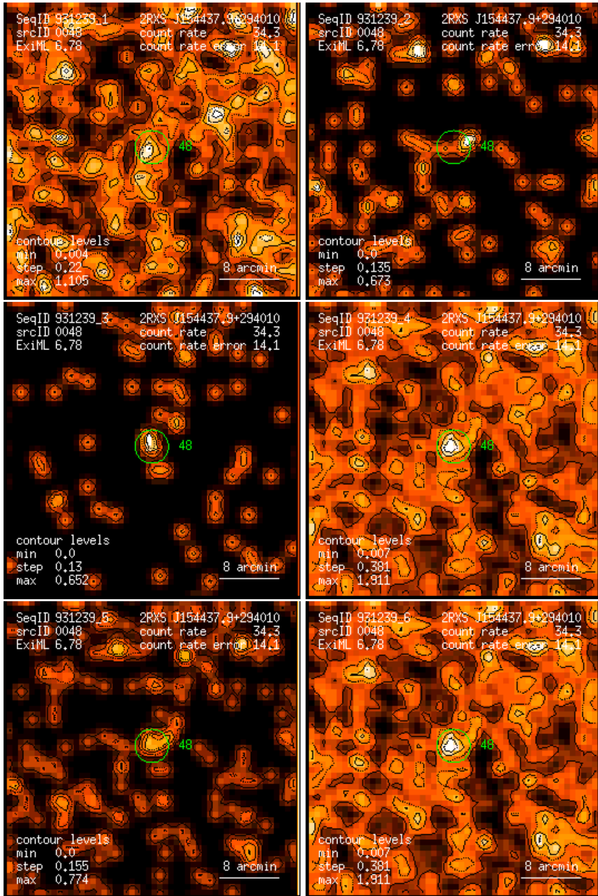
Figure 48: RASS 931239: detection 0048: band rate images, Gaussian filter: (1) PSPC channels 11 – 41, (2) 52 – 90, (3) 91 – 201, (4) 11 – 235, (5) 52 – 201, (6) 11 – 201. Broad band rates in counts/ks. Band rate contour levels in counts/ks/arcmin 2 .
