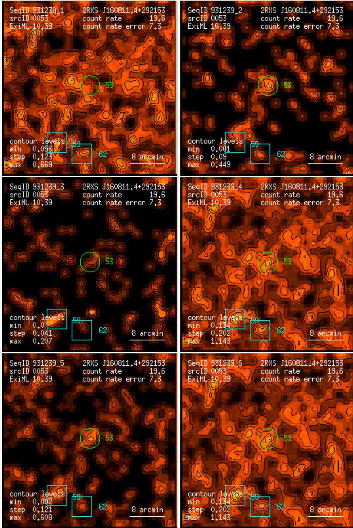
Figure 53: RASS 931239: detection 0053: band rate images, Gaussian filter: (1) PSPC channels 11 – 41, (2) 52 – 90, (3) 91 – 201, (4) 11 – 235, (5) 52 – 201, (6) 11 – 201. Broad band rates in counts/ks. Band rate contour levels in counts/ks/arcmin 2 .
