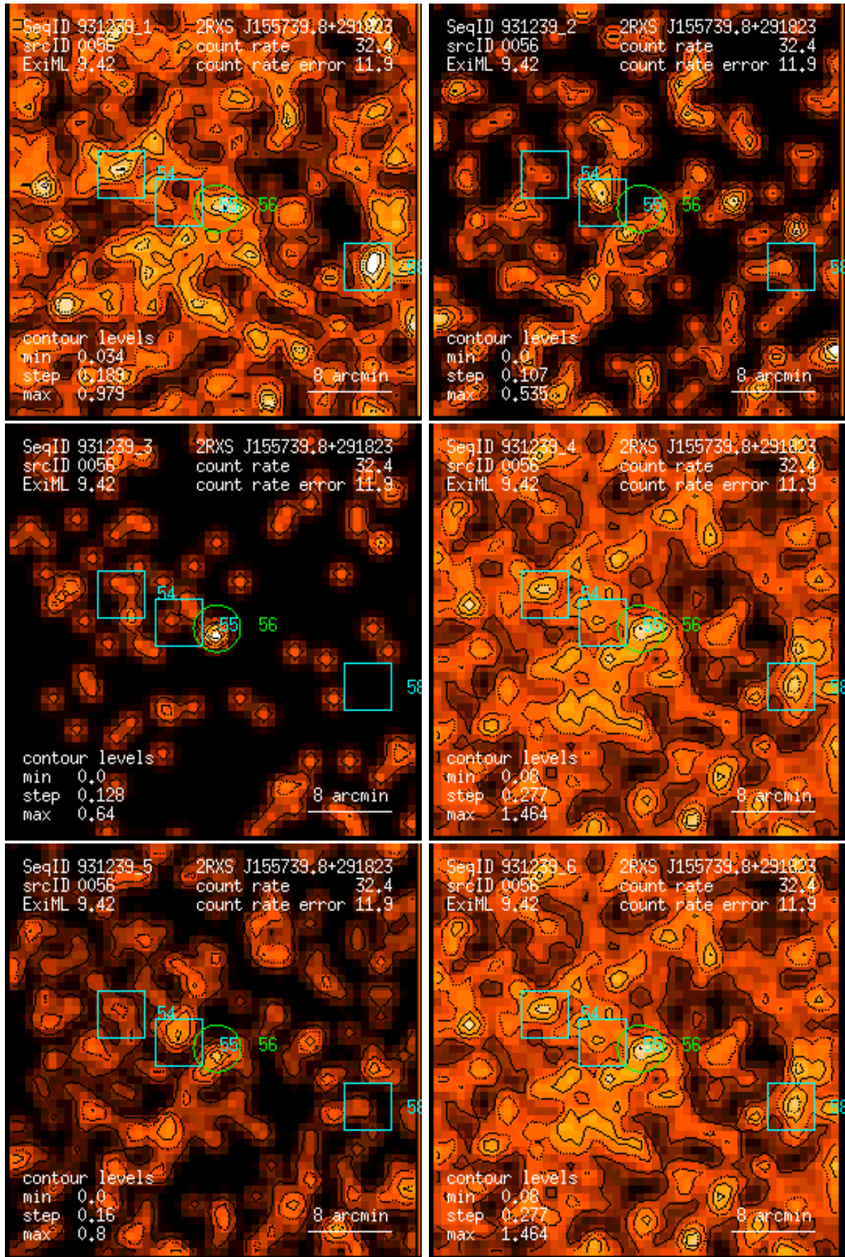
Figure 56: RASS 931239: detection 0056: band rate images, Gaussian filter: (1) PSPC channels 11 – 41, (2) 52 – 90, (3) 91 – 201, (4) 11 – 235, (5) 52 – 201, (6) 11 – 201. Broad band rates in counts/ks. Band rate contour levels in counts/ks/arcmin 2 .
