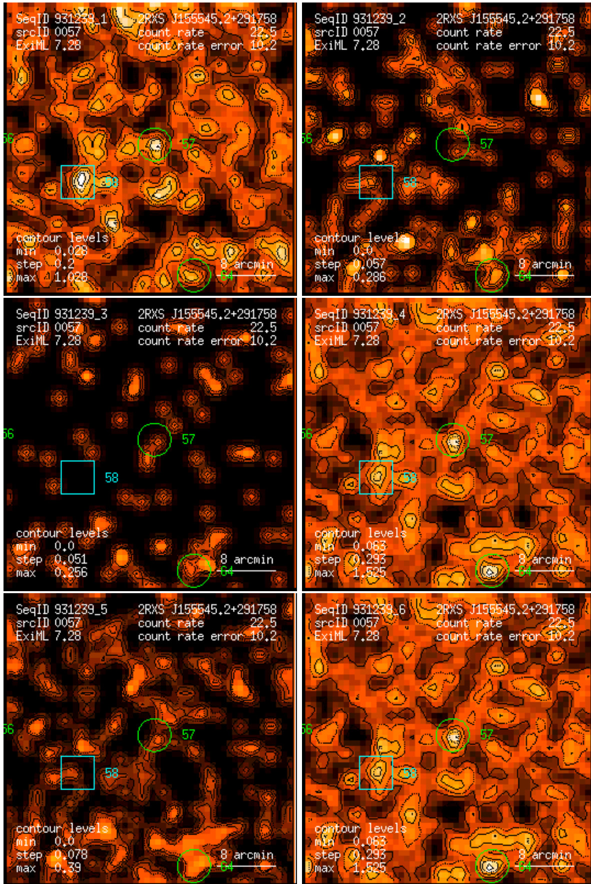
Figure 57: RASS 931239: detection 0057: band rate images, Gaussian filter: (1) PSPC channels 11 – 41, (2) 52 – 90, (3) 91 – 201, (4) 11 – 235, (5) 52 – 201, (6) 11 – 201. Broad band rates in counts/ks. Band rate contour levels in counts/ks/arcmin 2 .
