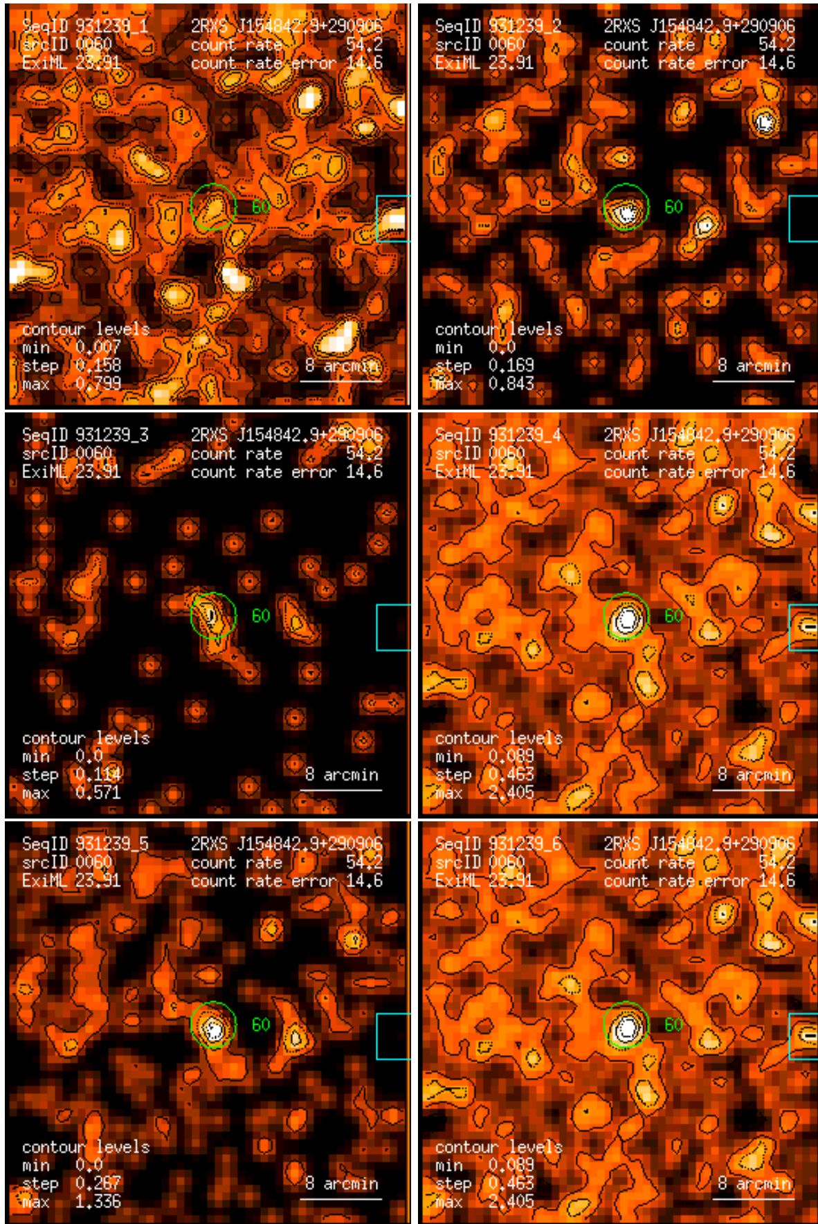
Figure 60: RASS 931239: detection 0060: band rate images, Gaussian filter: (1) PSPC channels 11 – 41, (2) 52 – 90, (3) 91 – 201, (4) 11 – 235, (5) 52 – 201, (6) 11 – 201. Broad band rates in counts/ks. Band rate contour levels in counts/ks/arcmin 2 .
