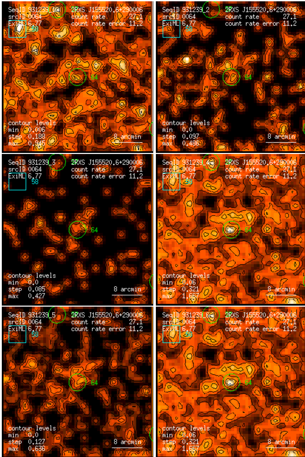
Figure 64: RASS 931239: detection 0064: band rate images, Gaussian filter: (1) PSPC channels 11 – 41, (2) 52 – 90, (3) 91 – 201, (4) 11 – 235, (5) 52 – 201, (6) 11 – 201. Broad band rates in counts/ks. Band rate contour levels in counts/ks/arcmin 2 .
