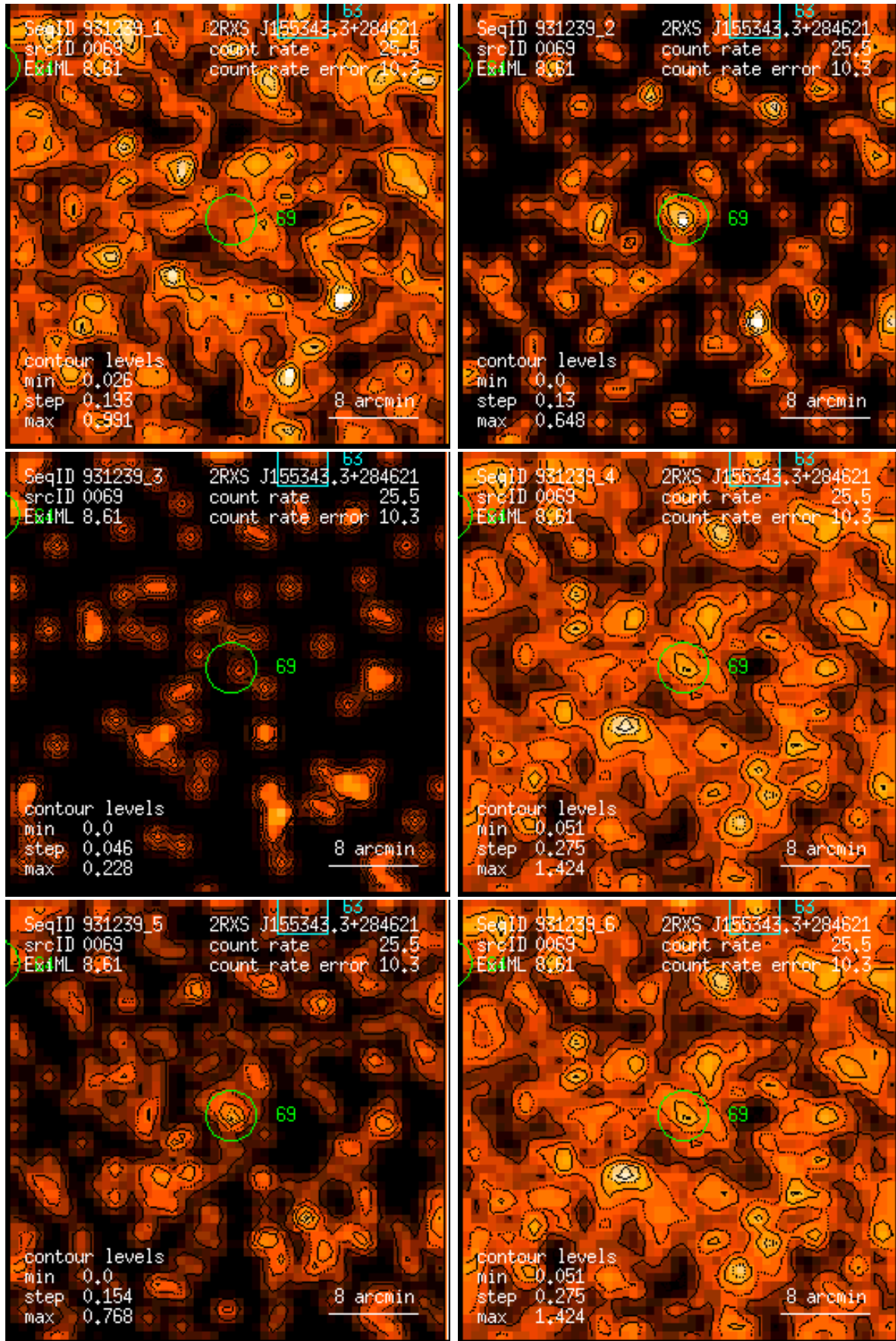
Figure 69: RASS 931239: detection 0069: band rate images, Gaussian filter: (1) PSPC channels 11 – 41, (2) 52 – 90, (3) 91 – 201, (4) 11 – 235, (5) 52 – 201, (6) 11 – 201. Broad band rates in counts/ks. Band rate contour levels in counts/ks/arcmin 2 .
