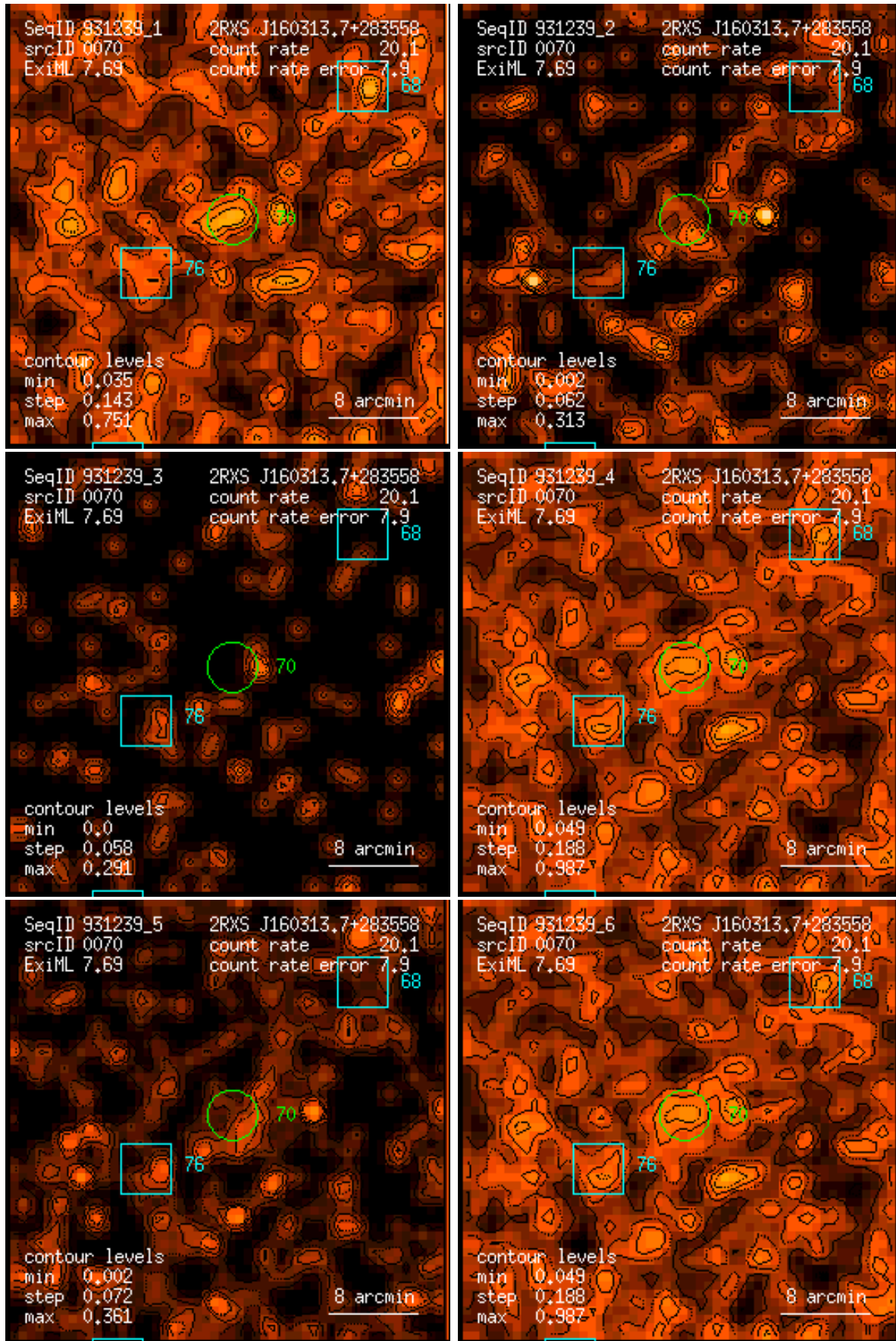
Figure 70: RASS 931239: detection 0070: band rate images, Gaussian filter: (1) PSPC channels 11 – 41, (2) 52 – 90, (3) 91 – 201, (4) 11 – 235, (5) 52 – 201, (6) 11 – 201. Broad band rates in counts/ks. Band rate contour levels in counts/ks/arcmin 2 .
