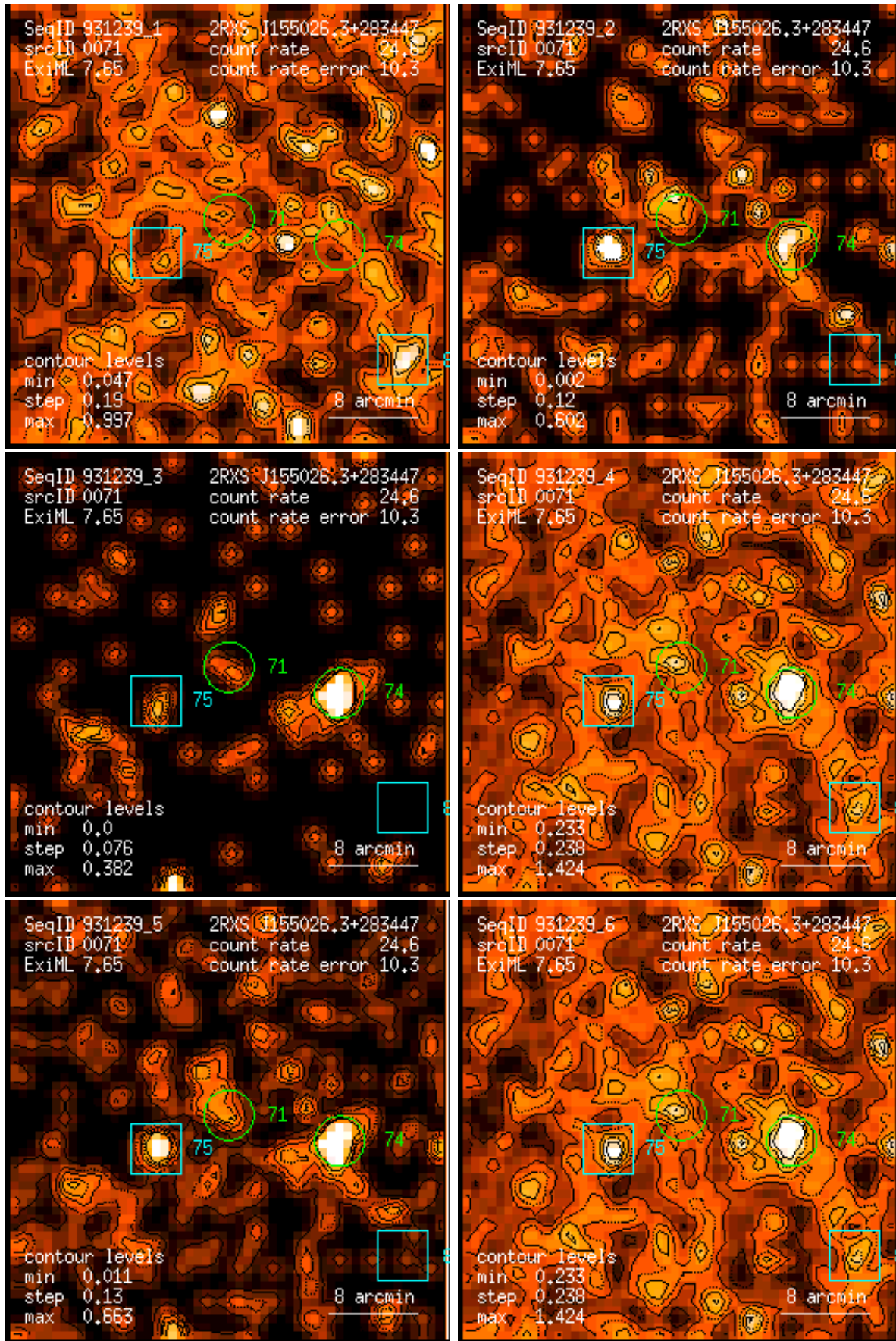
Figure 71: RASS 931239: detection 0071: band rate images, Gaussian filter: (1) PSPC channels 11 – 41, (2) 52 – 90, (3) 91 – 201, (4) 11 – 235, (5) 52 – 201, (6) 11 – 201. Broad band rates in counts/ks. Band rate contour levels in counts/ks/arcmin 2 .
