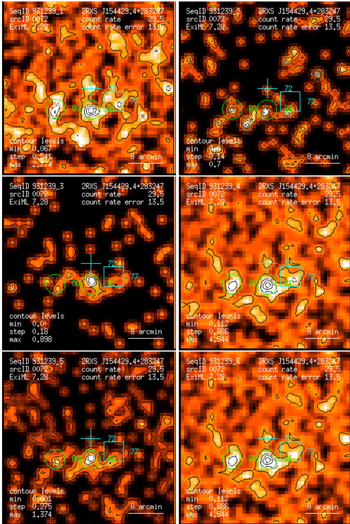
Figure 72: RASS 931239: detection 0072: band rate images, Gaussian filter: (1) PSPC channels 11 – 41, (2) 52 – 90, (3) 91 – 201, (4) 11 – 235, (5) 52 – 201, (6) 11 – 201. Broad band rates in counts/ks. Band rate contour levels in counts/ks/arcmin 2 .
