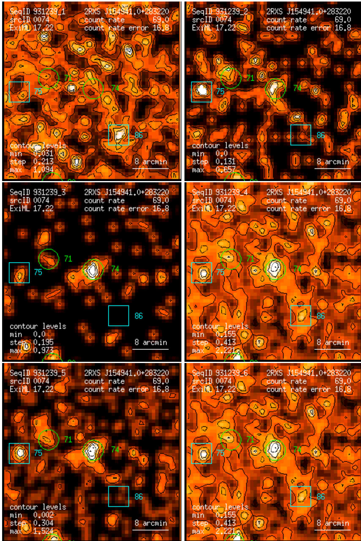
Figure 74: RASS 931239: detection 0074: band rate images, Gaussian filter: (1) PSPC channels 11 – 41, (2) 52 – 90, (3) 91 – 201, (4) 11 – 235, (5) 52 – 201, (6) 11 – 201. Broad band rates in counts/ks. Band rate contour levels in counts/ks/arcmin 2 .
