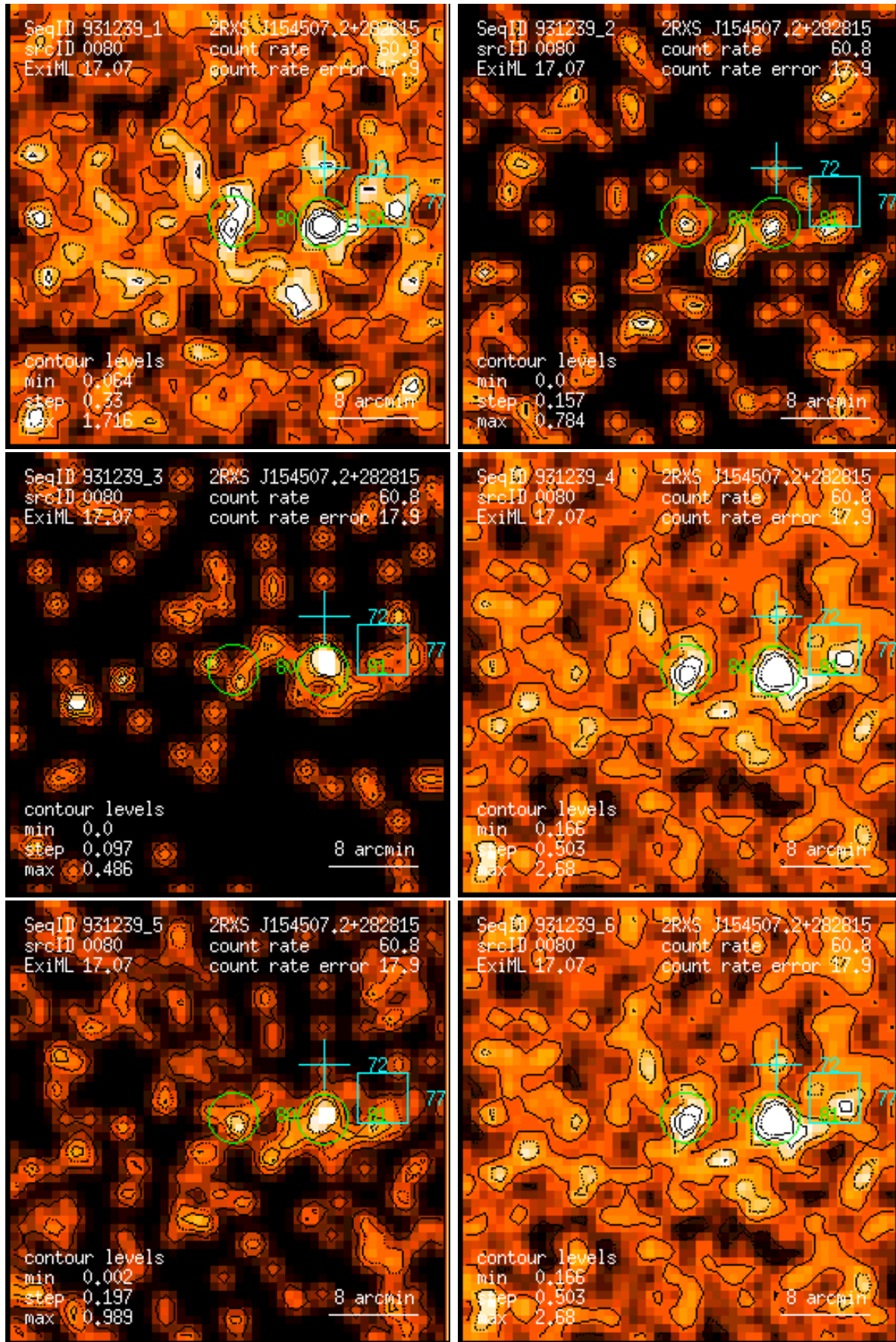
Figure 80: RASS 931239: detection 0080: band rate images, Gaussian filter: (1) PSPC channels 11 – 41, (2) 52 – 90, (3) 91 – 201, (4) 11 – 235, (5) 52 – 201, (6) 11 – 201. Broad band rates in counts/ks. Band rate contour levels in counts/ks/arcmin 2 .
