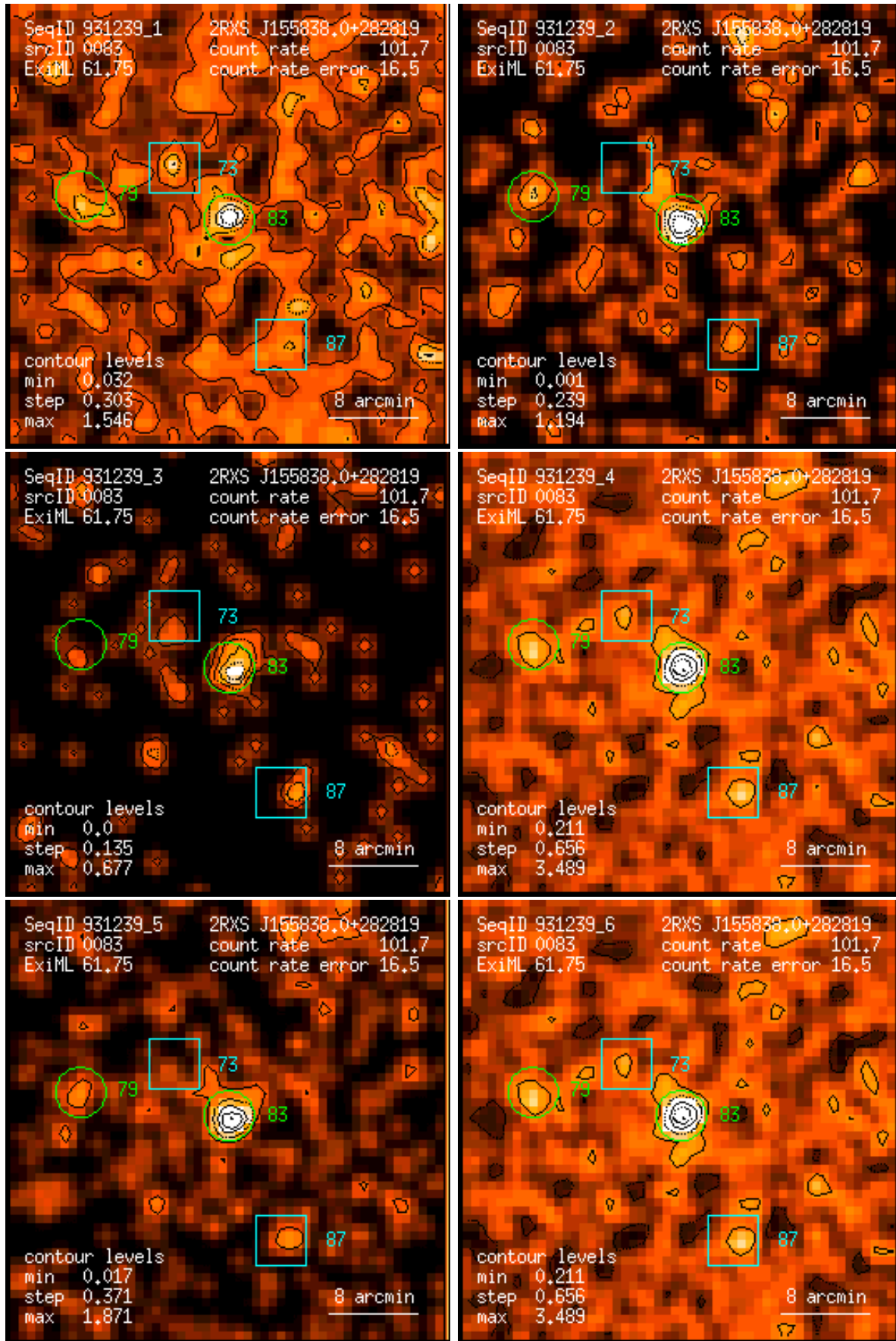
Figure 83: RASS 931239: detection 0083: band rate images, Gaussian filter: (1) PSPC channels 11 – 41, (2) 52 – 90, (3) 91 – 201, (4) 11 – 235, (5) 52 – 201, (6) 11 – 201. Broad band rates in counts/ks. Band rate contour levels in counts/ks/arcmin 2 .
