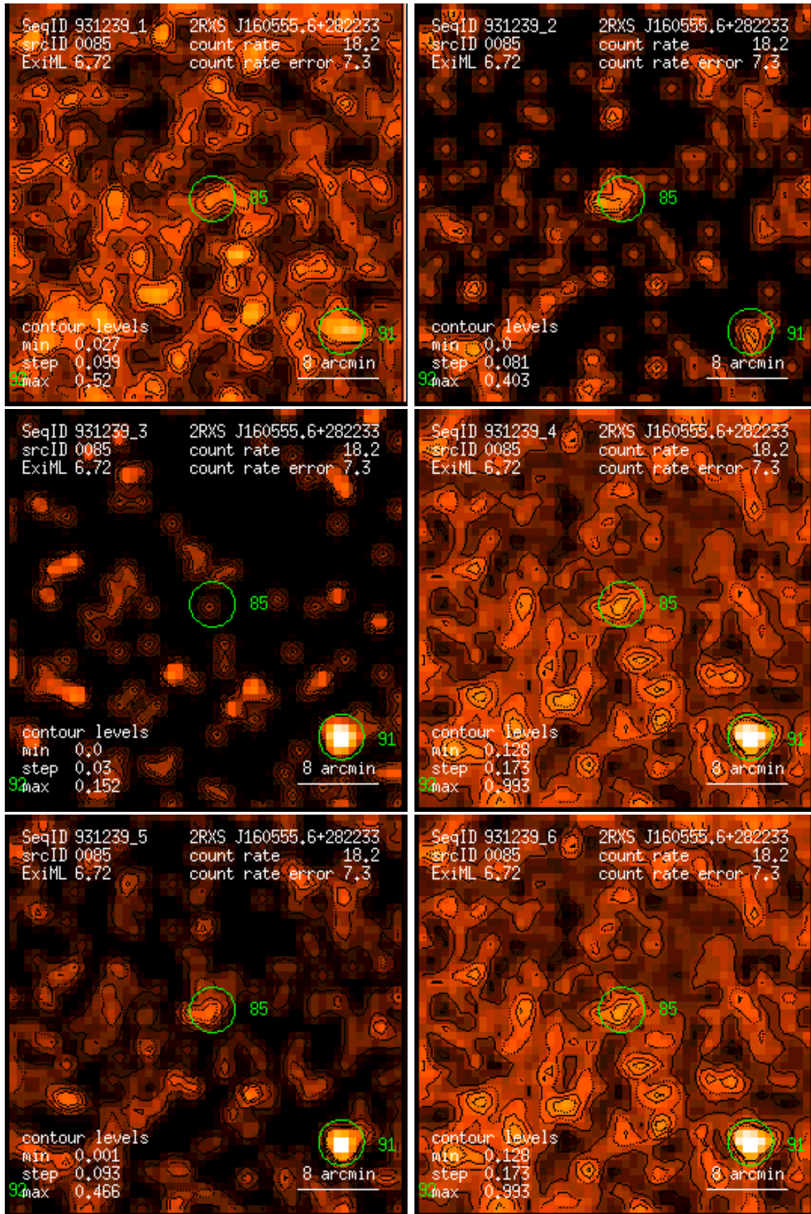
Figure 85: RASS 931239: detection 0085: band rate images, Gaussian filter: (1) PSPC channels 11 – 41, (2) 52 – 90, (3) 91 – 201, (4) 11 – 235, (5) 52 – 201, (6) 11 – 201. Broad band rates in counts/ks. Band rate contour levels in counts/ks/arcmin 2 .
