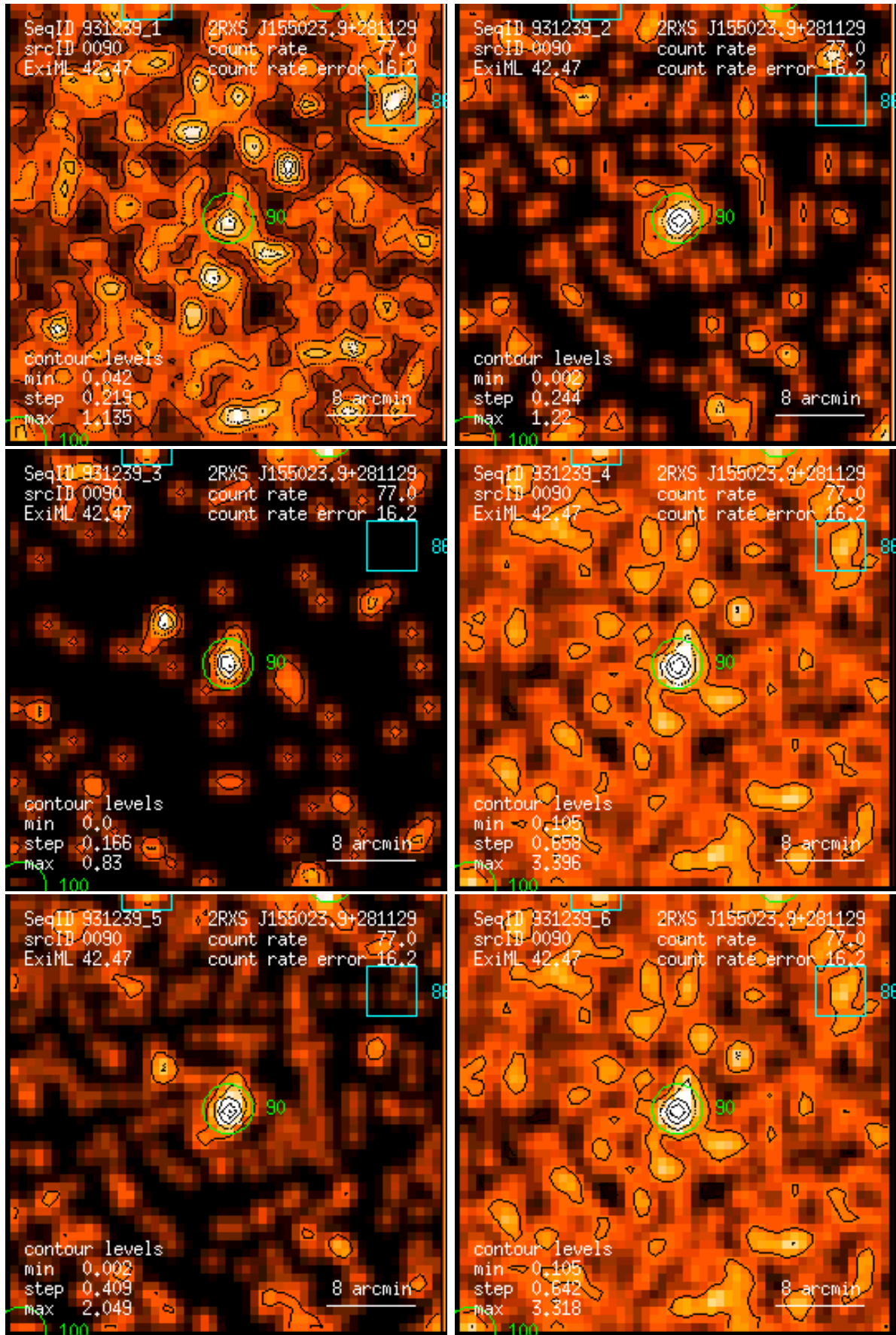
Figure 90: RASS 931239: detection 0090: band rate images, Gaussian filter: (1) PSPC channels 11 – 41, (2) 52 – 90, (3) 91 – 201, (4) 11 – 235, (5) 52 – 201, (6) 11 – 201. Broad band rates in counts/ks. Band rate contour levels in counts/ks/arcmin 2 .
