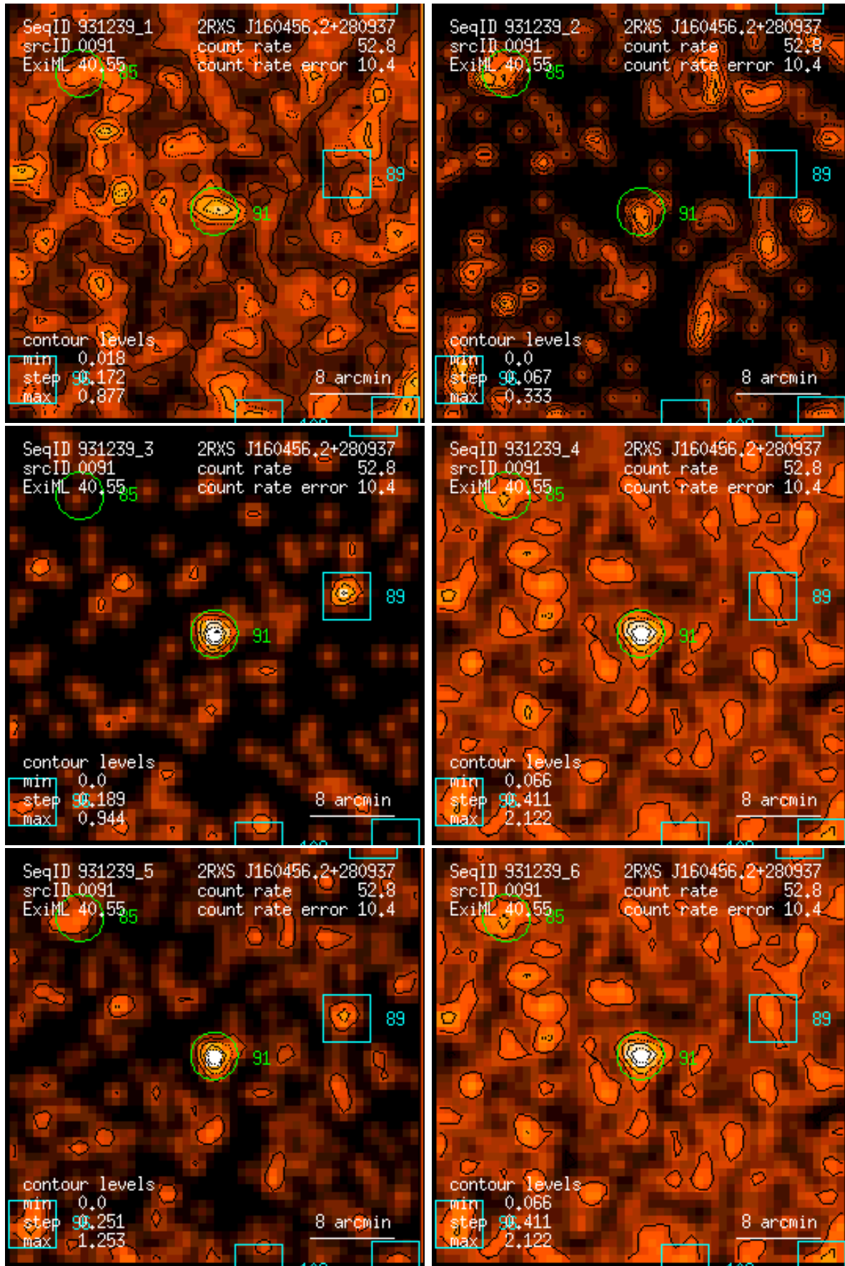
Figure 91: RASS 931239: detection 0091: band rate images, Gaussian filter: (1) PSPC channels 11 – 41, (2) 52 – 90, (3) 91 – 201, (4) 11 – 235, (5) 52 – 201, (6) 11 – 201. Broad band rates in counts/ks. Band rate contour levels in counts/ks/arcmin 2 .
