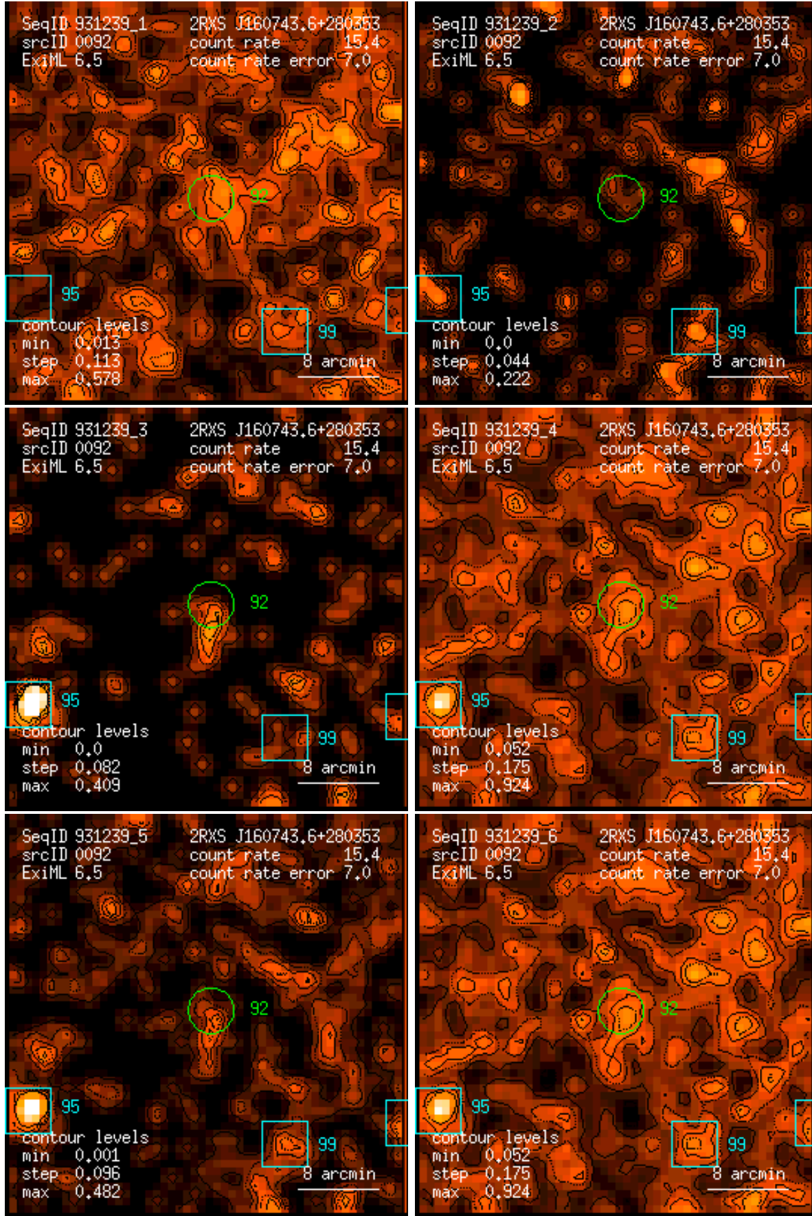
Figure 92: RASS 931239: detection 0092: band rate images, Gaussian filter: (1) PSPC channels 11 – 41, (2) 52 – 90, (3) 91 – 201, (4) 11 – 235, (5) 52 – 201, (6) 11 – 201. Broad band rates in counts/ks. Band rate contour levels in counts/ks/arcmin 2 .
