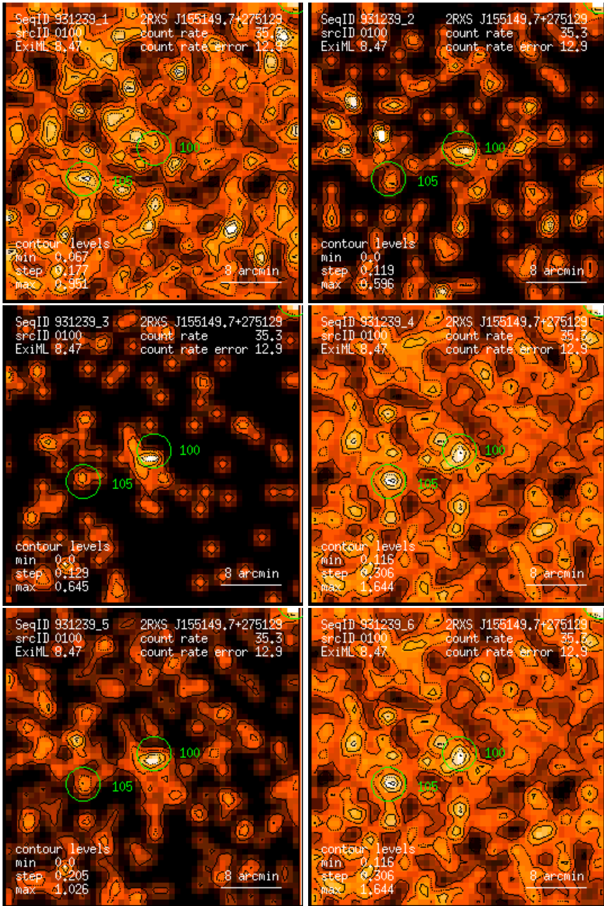
Figure 100: RASS 931239: detection 0100: band rate images, Gaussian filter: (1) PSPC channels 11 – 41, (2) 52 – 90, (3) 91 – 201, (4) 11 – 235, (5) 52 – 201, (6) 11 – 201. Broad band rates in counts/ks. Band rate contour levels in counts/ks/arcmin 2 .
