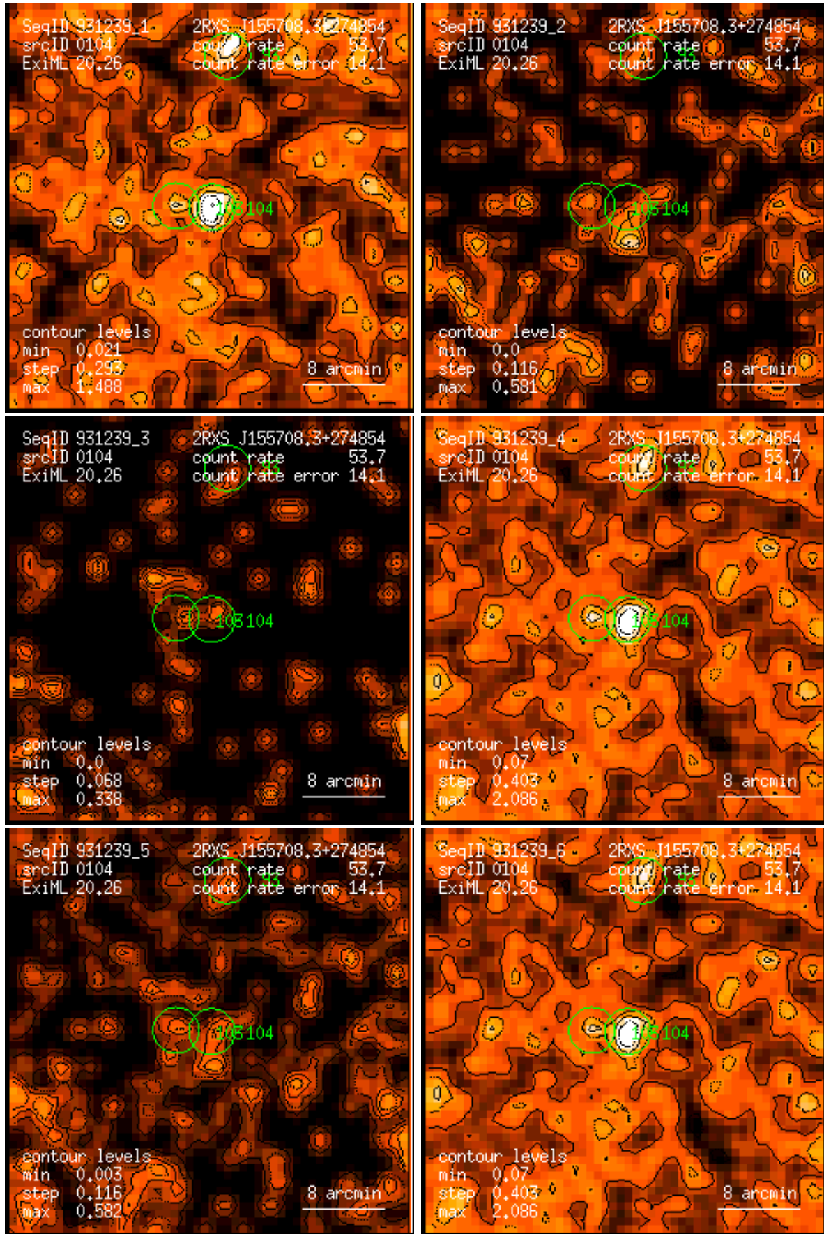
Figure 104: RASS 931239: detection 0104: band rate images, Gaussian filter: (1) PSPC channels 11 – 41, (2) 52 – 90, (3) 91 – 201, (4) 11 – 235, (5) 52 – 201, (6) 11 – 201. Broad band rates in counts/ks. Band rate contour levels in counts/ks/arcmin 2 .
