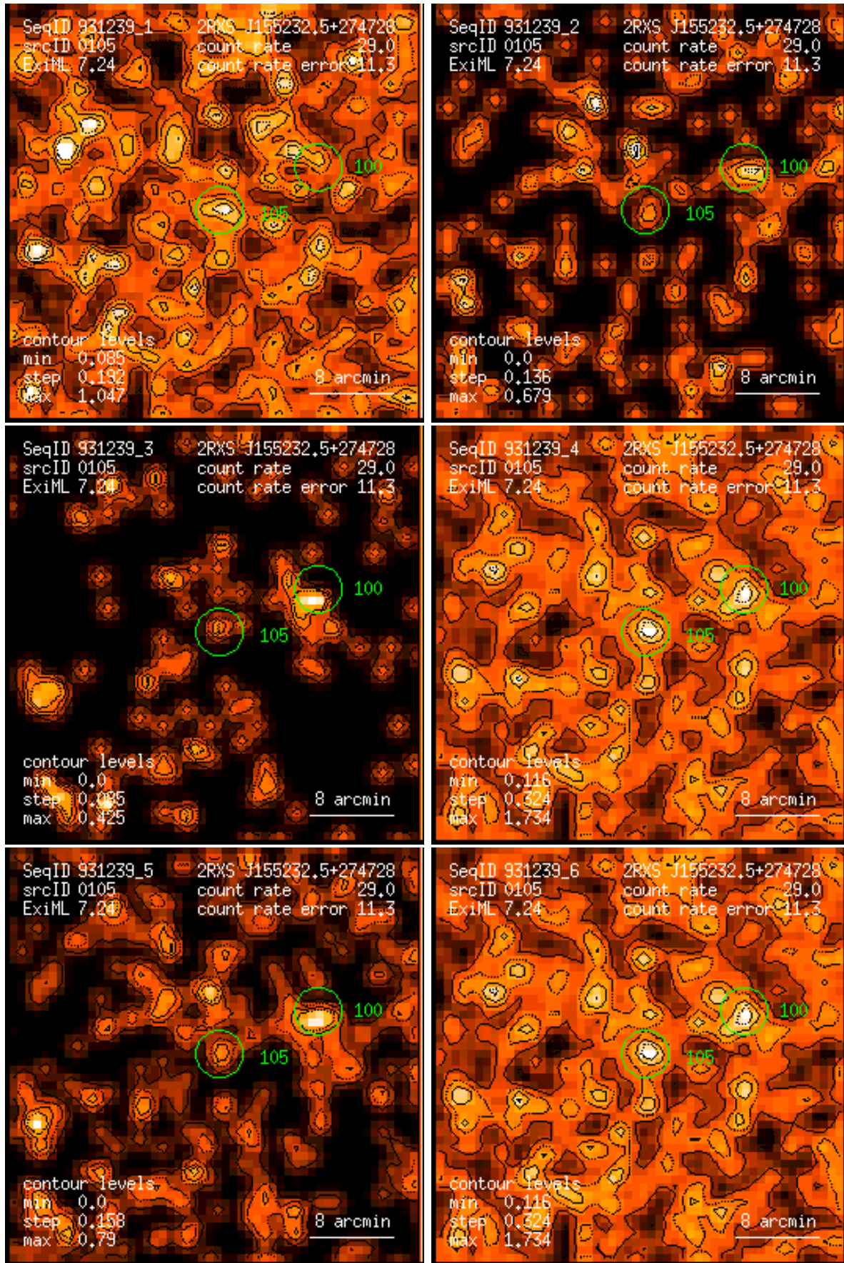
Figure 105: RASS 931239: detection 0105: band rate images, Gaussian filter: (1) PSPC channels 11 – 41, (2) 52 – 90, (3) 91 – 201, (4) 11 – 235, (5) 52 – 201, (6) 11 – 201. Broad band rates in counts/ks. Band rate contour levels in counts/ks/arcmin 2 .
