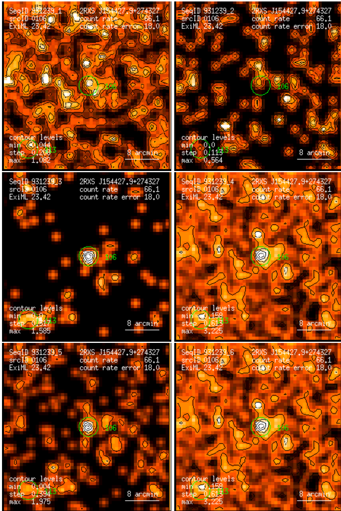
Figure 106: RASS 931239: detection 0106: band rate images, Gaussian filter: (1) PSPC channels 11 – 41, (2) 52 – 90, (3) 91 – 201, (4) 11 – 235, (5) 52 – 201, (6) 11 – 201. Broad band rates in counts/ks. Band rate contour levels in counts/ks/arcmin 2 .
