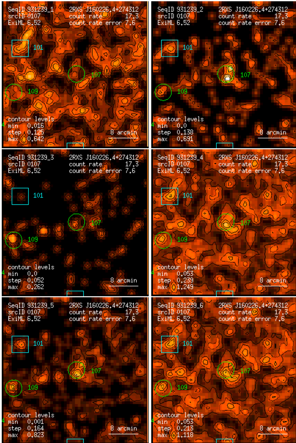
Figure 107: RASS 931239: detection 0107: band rate images, Gaussian filter: (1) PSPC channels 11 – 41, (2) 52 – 90, (3) 91 – 201, (4) 11 – 235, (5) 52 – 201, (6) 11 – 201. Broad band rates in counts/ks. Band rate contour levels in counts/ks/arcmin 2 .
