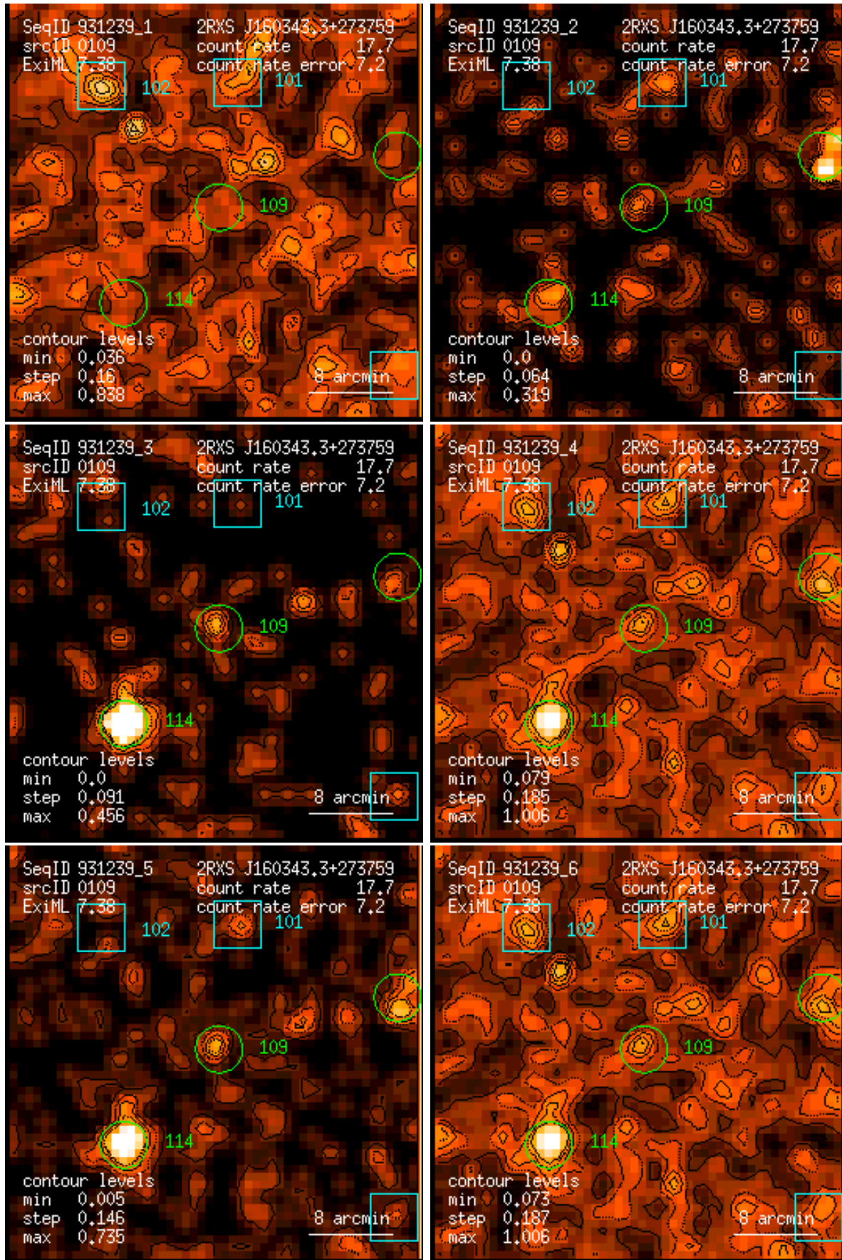
Figure 109: RASS 931239: detection 0109: band rate images, Gaussian filter: (1) PSPC channels 11 – 41, (2) 52 – 90, (3) 91 – 201, (4) 11 – 235, (5) 52 – 201, (6) 11 – 201. Broad band rates in counts/ks. Band rate contour levels in counts/ks/arcmin 2 .
