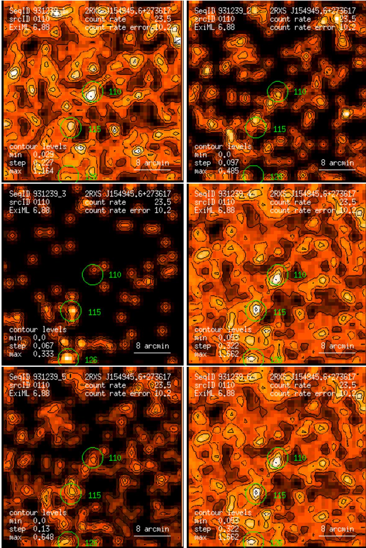
Figure 110: RASS 931239: detection 0110: band rate images, Gaussian filter: (1) PSPC channels 11 – 41, (2) 52 – 90, (3) 91 – 201, (4) 11 – 235, (5) 52 – 201, (6) 11 – 201. Broad band rates in counts/ks. Band rate contour levels in counts/ks/arcmin 2 .
