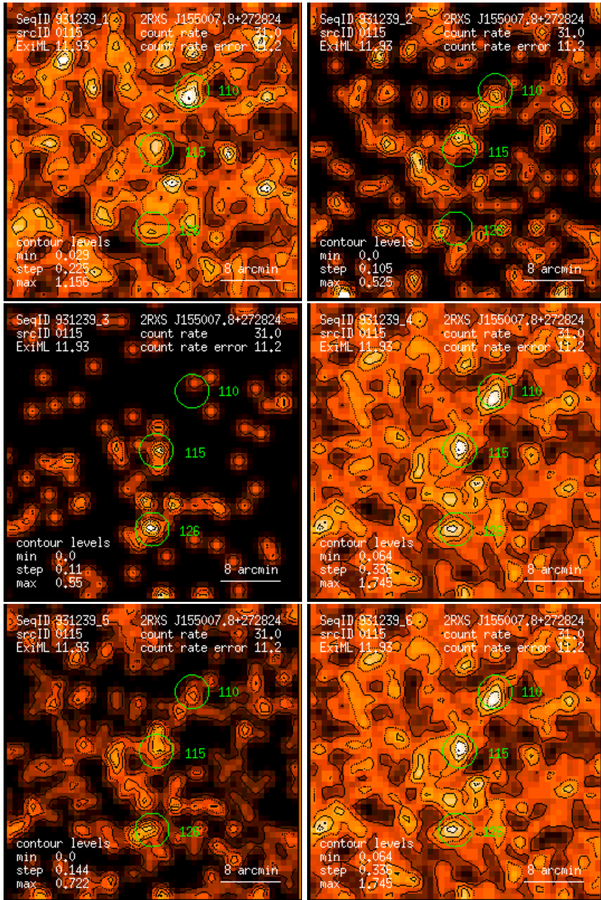
Figure 115: RASS 931239: detection 0115: band rate images, Gaussian filter: (1) PSPC channels 11 – 41, (2) 52 – 90, (3) 91 – 201, (4) 11 – 235, (5) 52 – 201, (6) 11 – 201. Broad band rates in counts/ks. Band rate contour levels in counts/ks/arcmin 2 .
