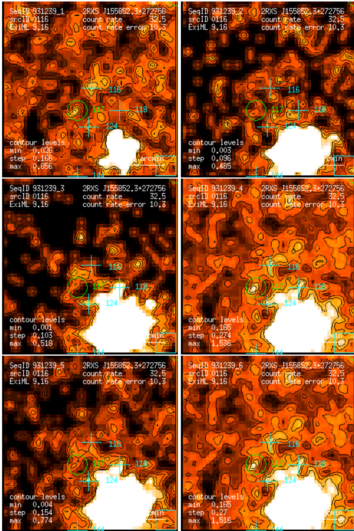
Figure 116: RASS 931239: detection 0116: band rate images, Gaussian filter: (1) PSPC channels 11 – 41, (2) 52 – 90, (3) 91 – 201, (4) 11 – 235, (5) 52 – 201, (6) 11 – 201. Broad band rates in counts/ks. Band rate contour levels in counts/ks/arcmin 2 .
