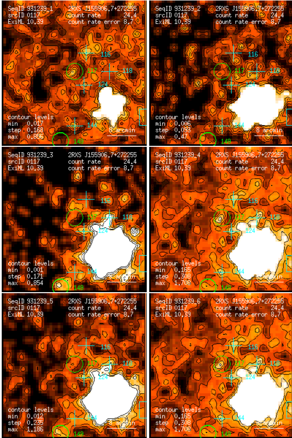
Figure 117: RASS 931239: detection 0117: band rate images, Gaussian filter: (1) PSPC channels 11 – 41, (2) 52 – 90, (3) 91 – 201, (4) 11 – 235, (5) 52 – 201, (6) 11 – 201. Broad band rates in counts/ks. Band rate contour levels in counts/ks/arcmin 2 .
