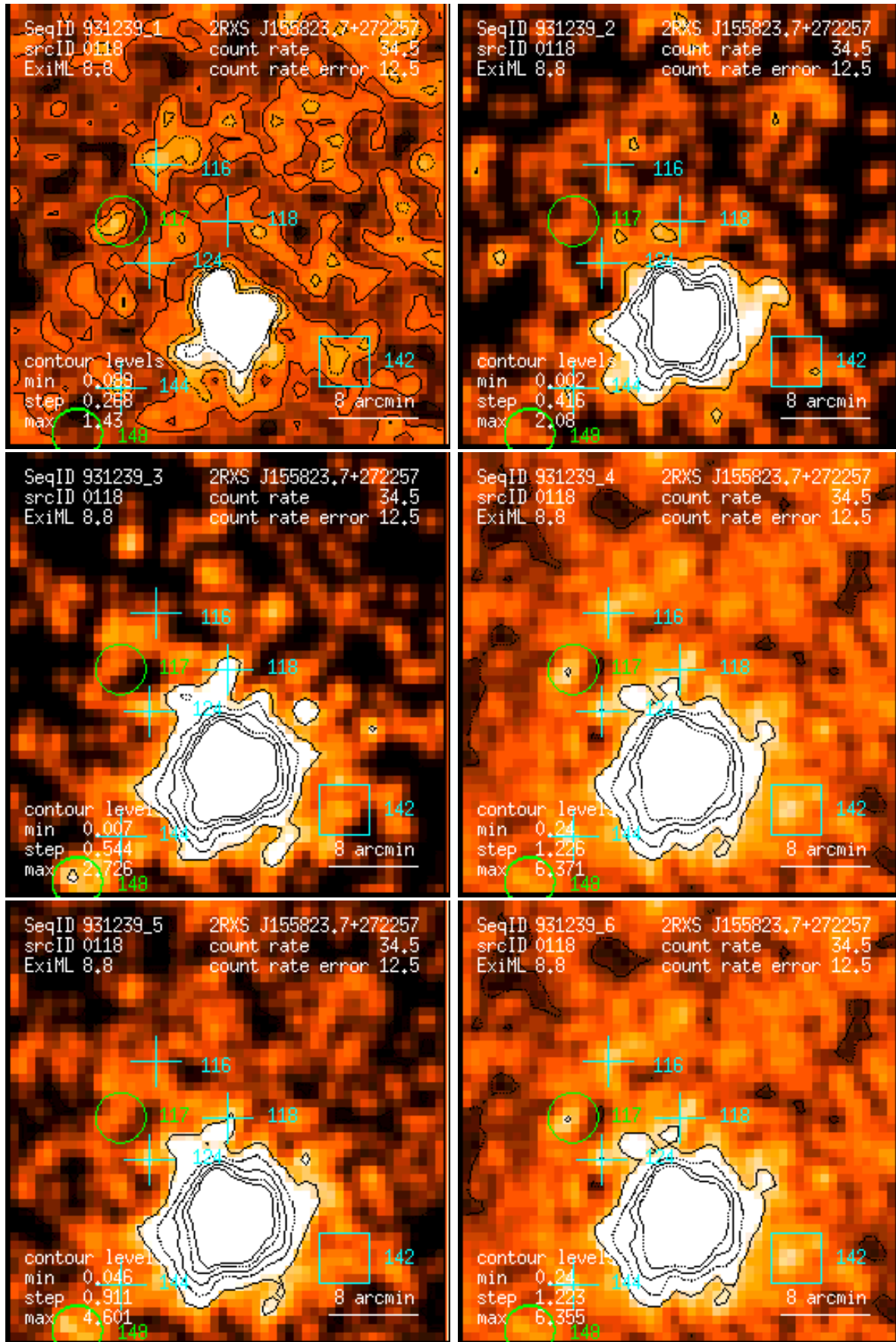
Figure 118: RASS 931239: detection 0118: band rate images, Gaussian filter: (1) PSPC channels 11 – 41, (2) 52 – 90, (3) 91 – 201, (4) 11 – 235, (5) 52 – 201, (6) 11 – 201. Broad band rates in counts/ks. Band rate contour levels in counts/ks/arcmin 2 .
