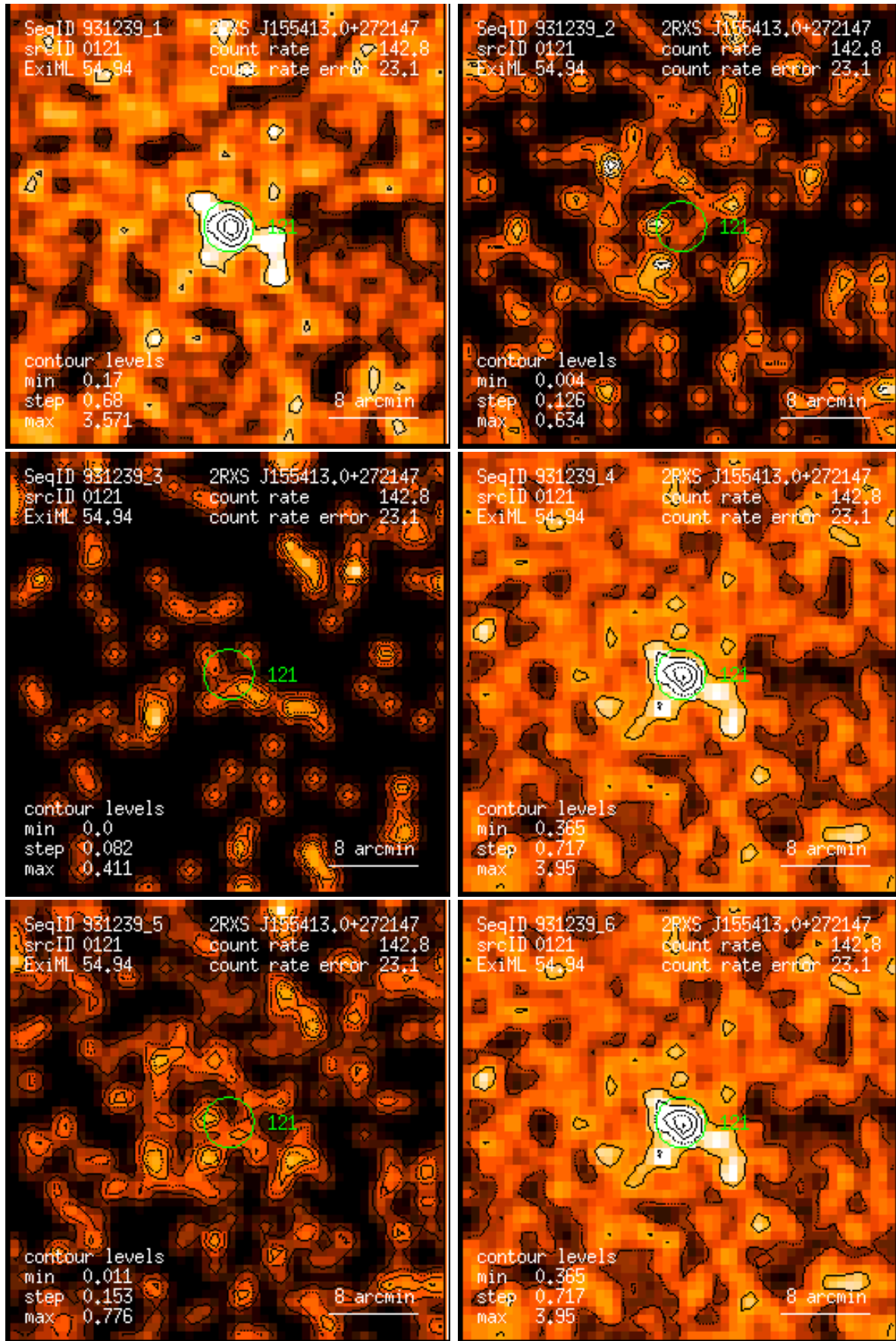
Figure 121: RASS 931239: detection 0121: band rate images, Gaussian filter: (1) PSPC channels 11 – 41, (2) 52 – 90, (3) 91 – 201, (4) 11 – 235, (5) 52 – 201, (6) 11 – 201. Broad band rates in counts/ks. Band rate contour levels in counts/ks/arcmin 2 .
