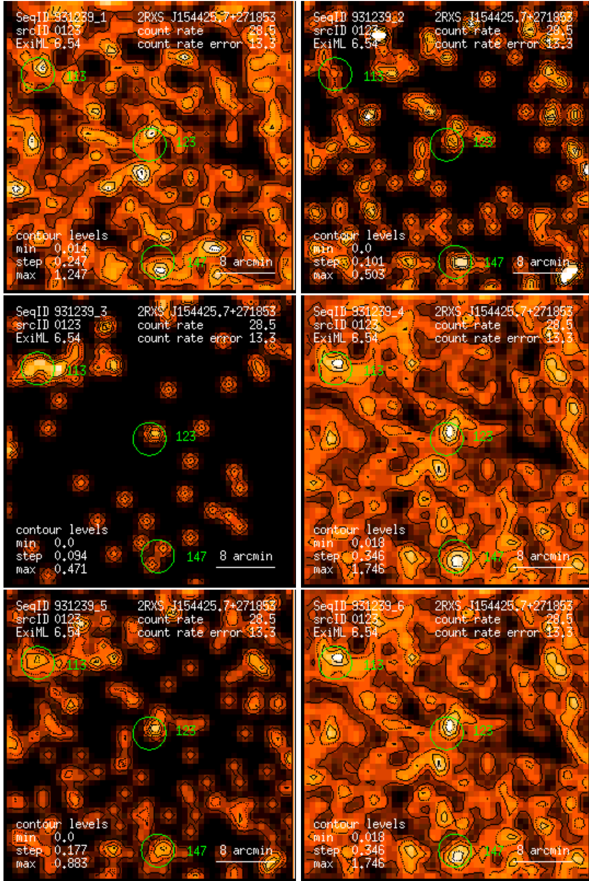
Figure 123: RASS 931239: detection 0123: band rate images, Gaussian filter: (1) PSPC channels 11 – 41, (2) 52 – 90, (3) 91 – 201, (4) 11 – 235, (5) 52 – 201, (6) 11 – 201. Broad band rates in counts/ks. Band rate contour levels in counts/ks/arcmin 2 .
