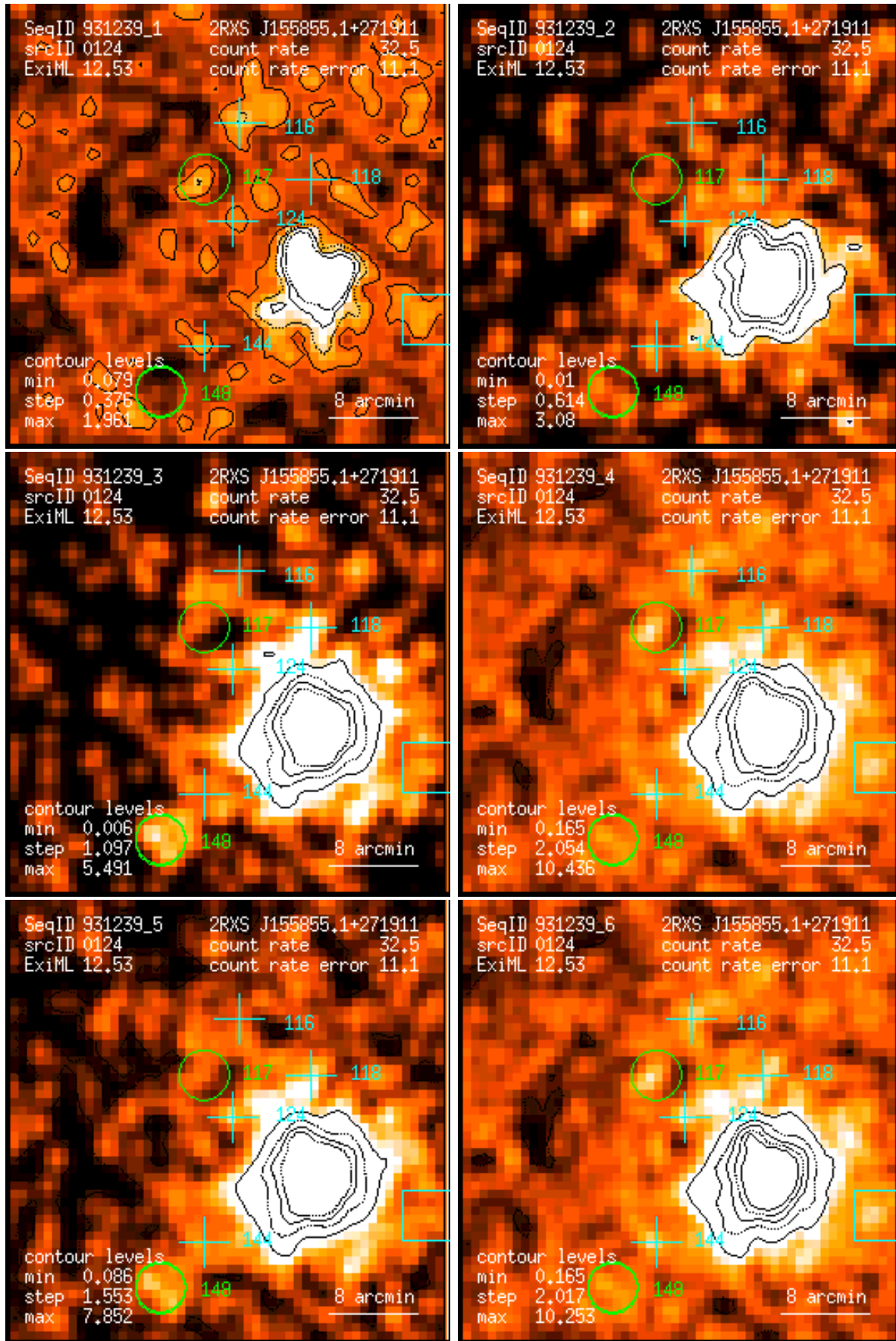
Figure 124: RASS 931239: detection 0124: band rate images, Gaussian filter: (1) PSPC channels 11 – 41, (2) 52 – 90, (3) 91 – 201, (4) 11 – 235, (5) 52 – 201, (6) 11 – 201. Broad band rates in counts/ks. Band rate contour levels in counts/ks/arcmin 2 .
