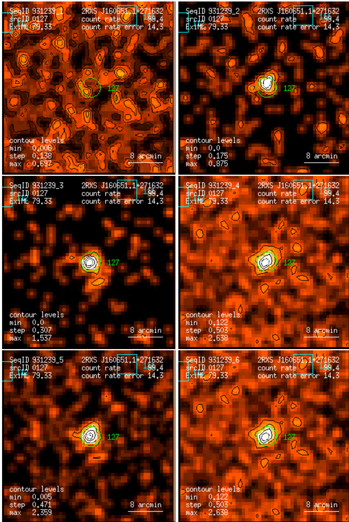
Figure 127: RASS 931239: detection 0127: band rate images, Gaussian filter: (1) PSPC channels 11 – 41, (2) 52 – 90, (3) 91 – 201, (4) 11 – 235, (5) 52 – 201, (6) 11 – 201. Broad band rates in counts/ks. Band rate contour levels in counts/ks/arcmin 2 .
