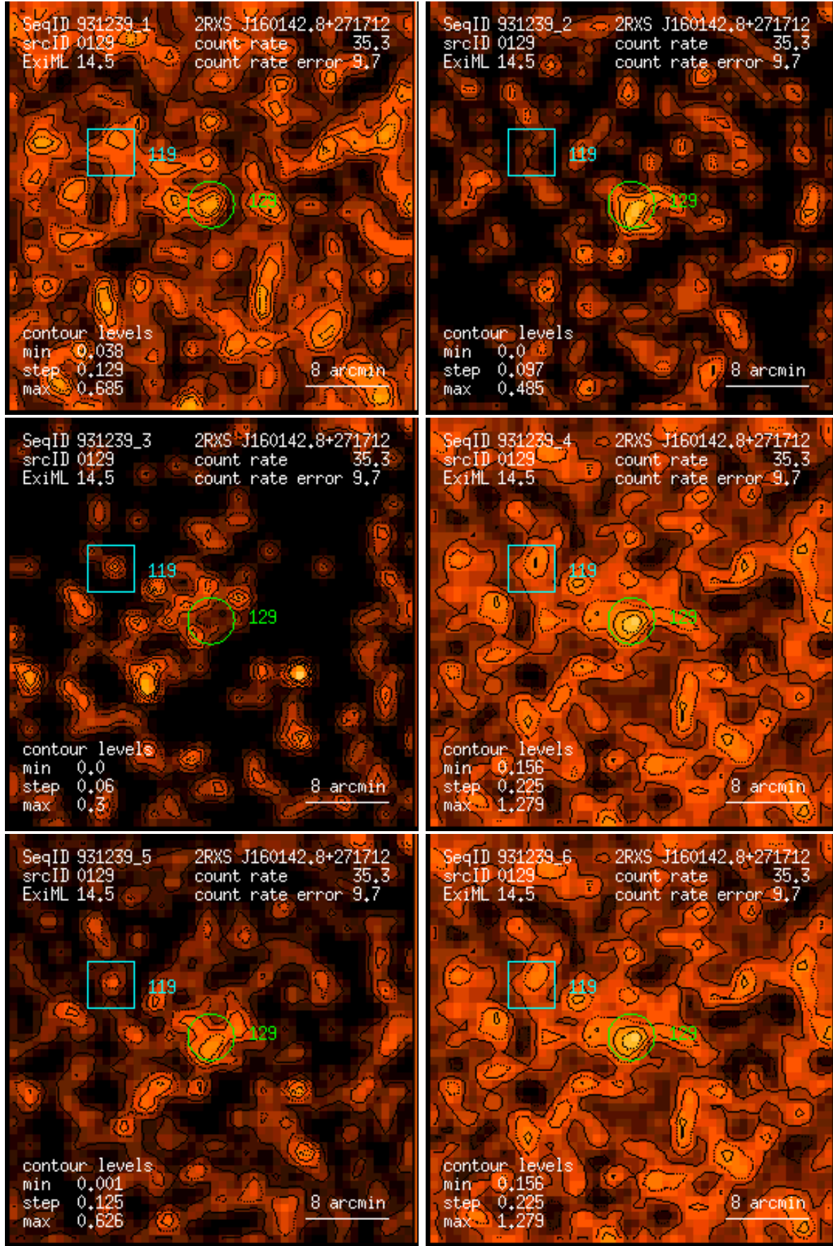
Figure 129: RASS 931239: detection 0129: band rate images, Gaussian filter: (1) PSPC channels 11 – 41, (2) 52 – 90, (3) 91 – 201, (4) 11 – 235, (5) 52 – 201, (6) 11 – 201. Broad band rates in counts/ks. Band rate contour levels in counts/ks/arcmin 2 .
